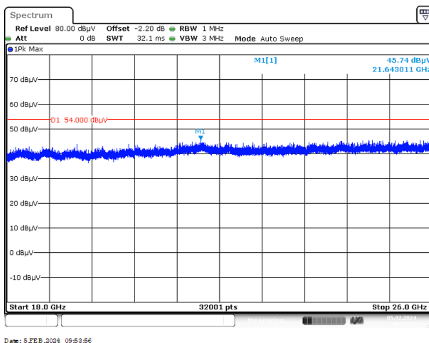
Plot 4: 18 GHz to 26 GHz, vertical & horizontal polarization, valid for all channels and modes
