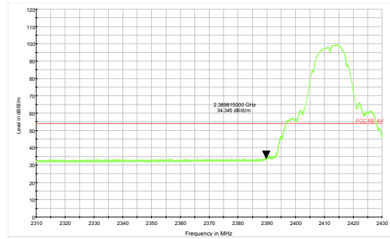
802.11b-Channel 1 Average
