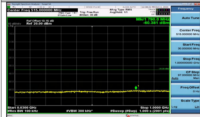
Band41_15MHz_16QAM_40740_1RB#0_30~1000_30~1000 00
