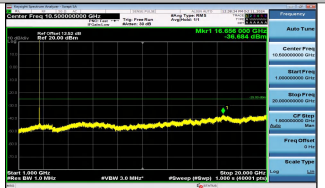
Band41_15MHz_16QAM_40740_1RB#0_1000~20000_1000~20000 00~20000
