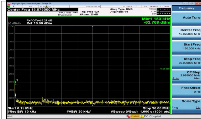
Band41_15MHz_QPSK_40740_1RB#0_0.15~30_0.15~30
