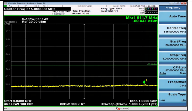
Band41_15MHz_QPSK_40740_1RB#0_30~1000_30~1000 0
