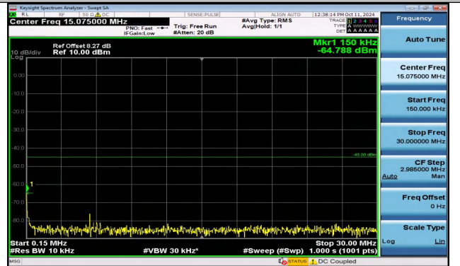
Band41_15MHz_16QAM_40740_1RB#0_0.15~30_0.15~30 0
