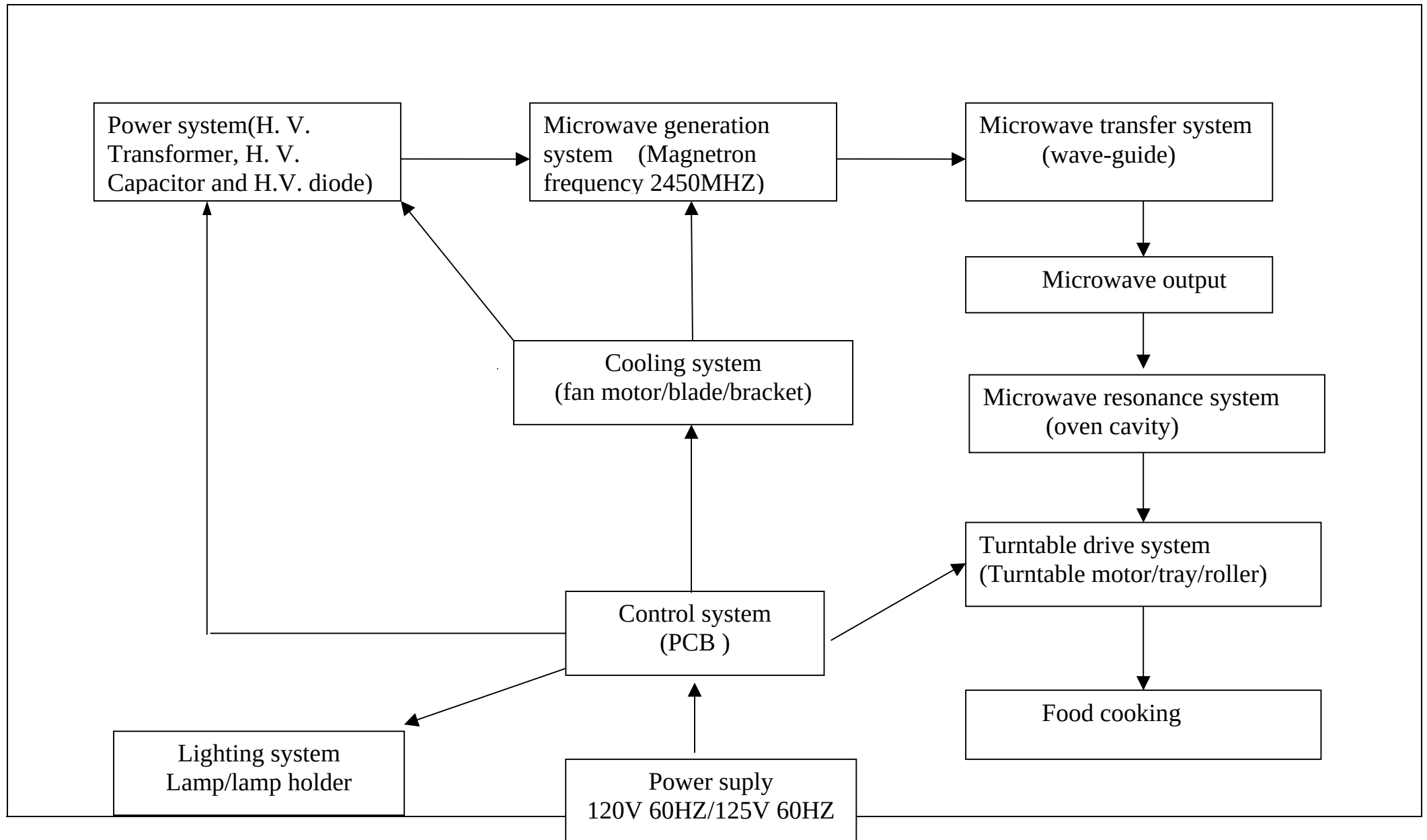
EM920AFW-P block diagram
