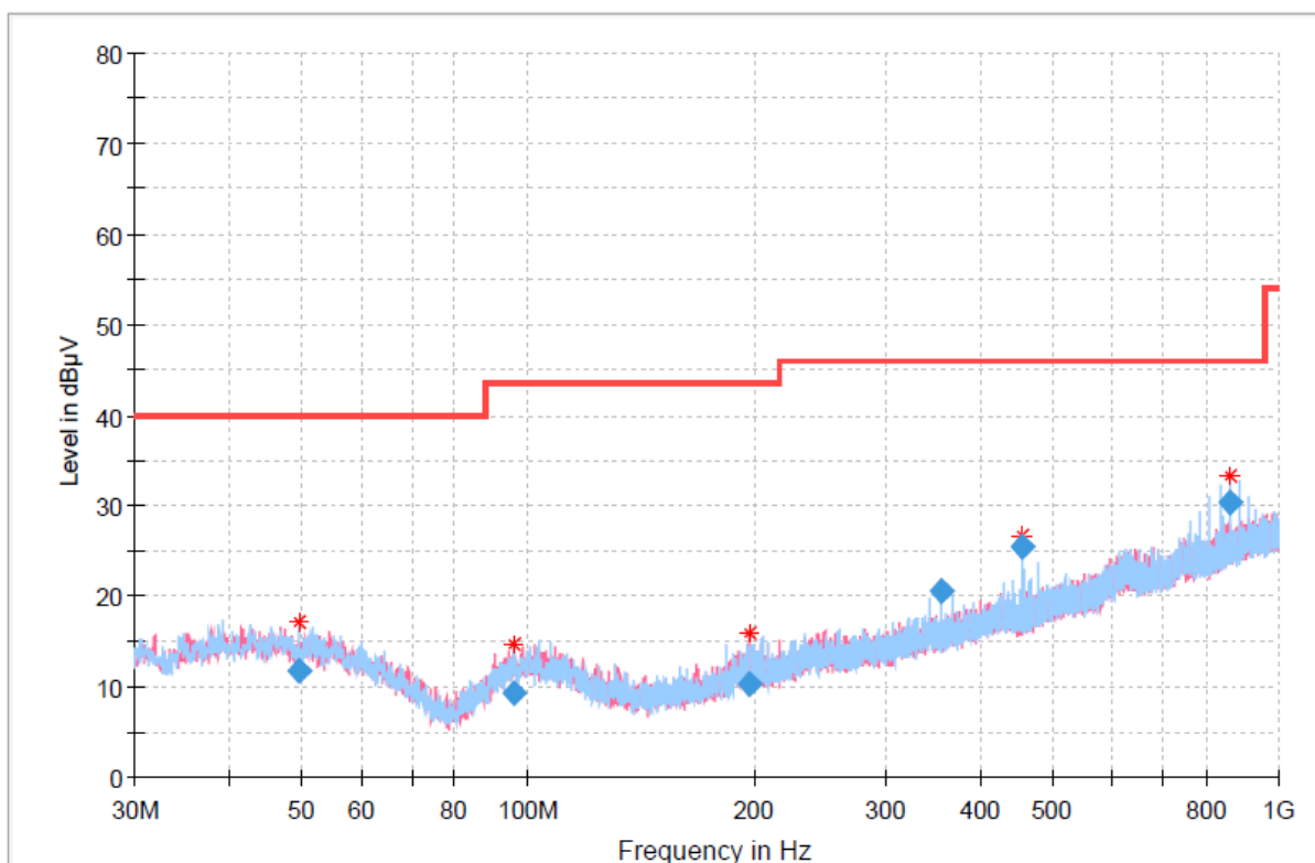
Worst case – RSE (Below 1 GHz)_2.4GHz_ANT 1
