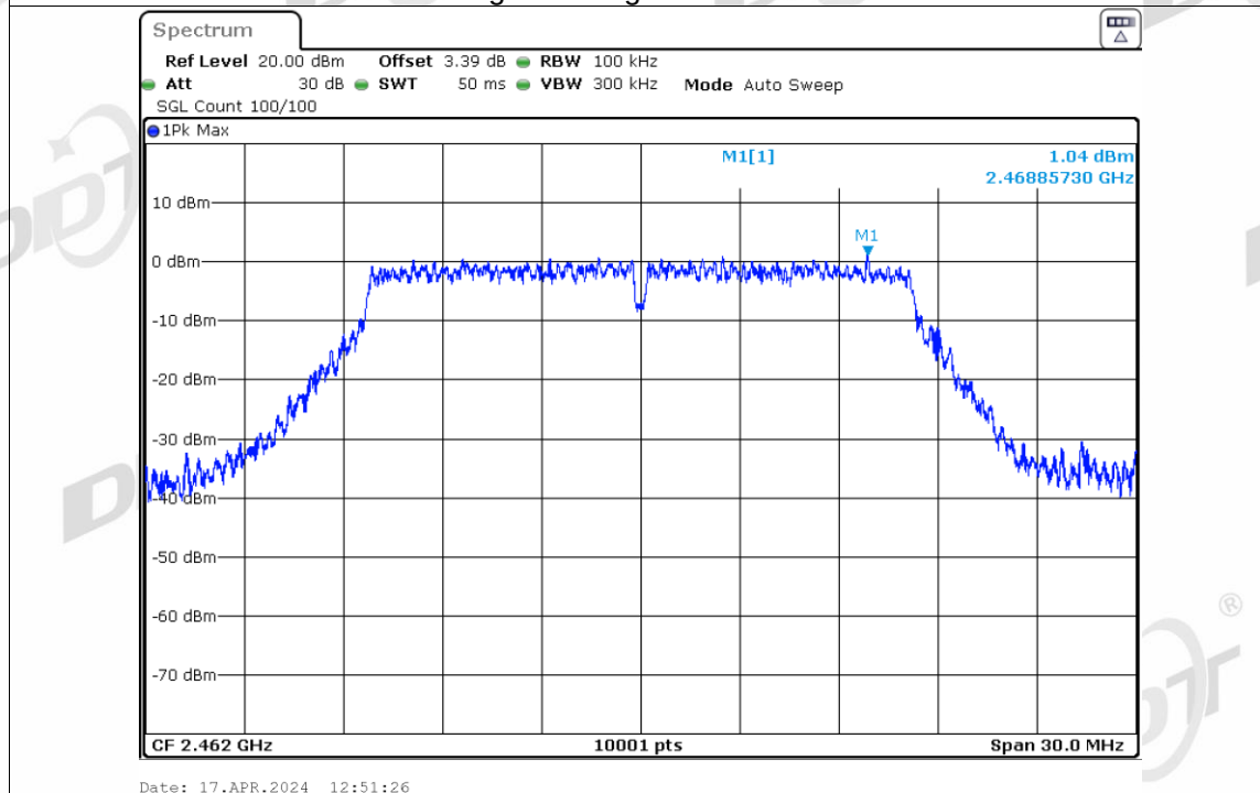
Band Edge NVNT g 2462MHz Ant1 Emission
