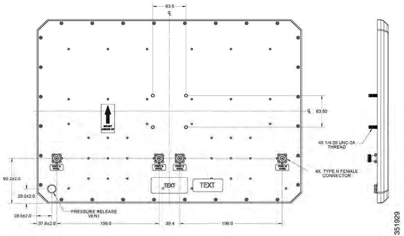
Figure 3 Rear View of Antenna (dimensions in millimeters)
