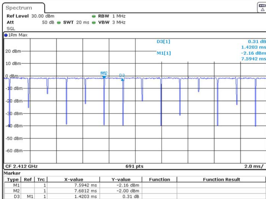
Test Graph_IEEE802.11g Duty Cycle:
