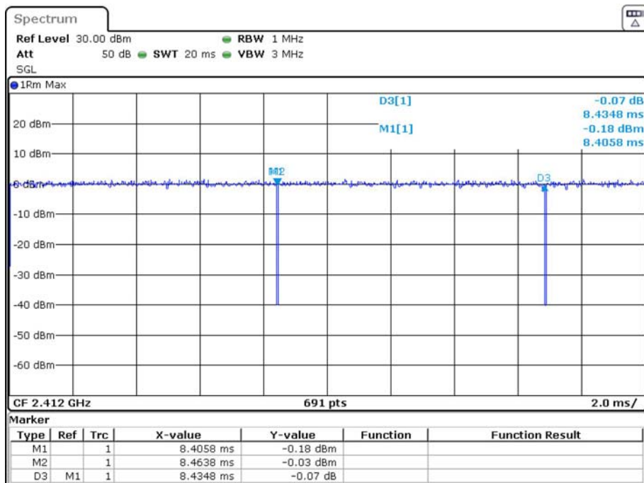
Test Graph_IEEE802.11b Duty Cycle:
