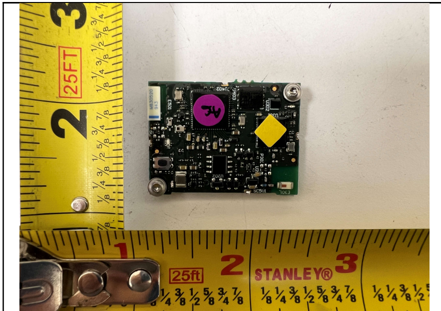
Module Uncover View
