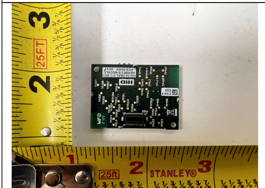
Module Rear View
