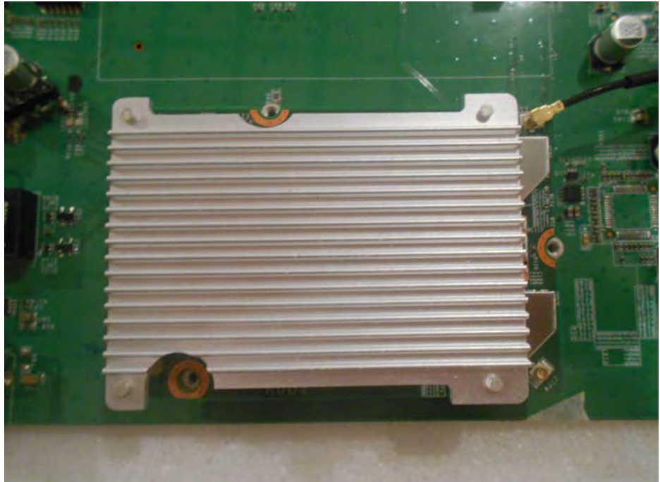
CLOSE-UP VIEW
