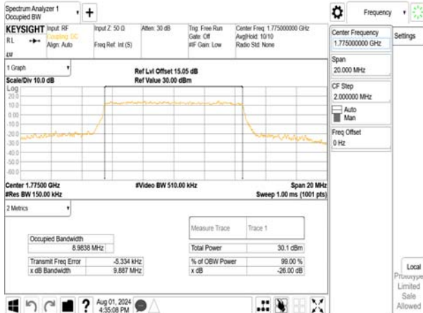
Band66_10MHz_64QAM_RB50_0_CH132622
