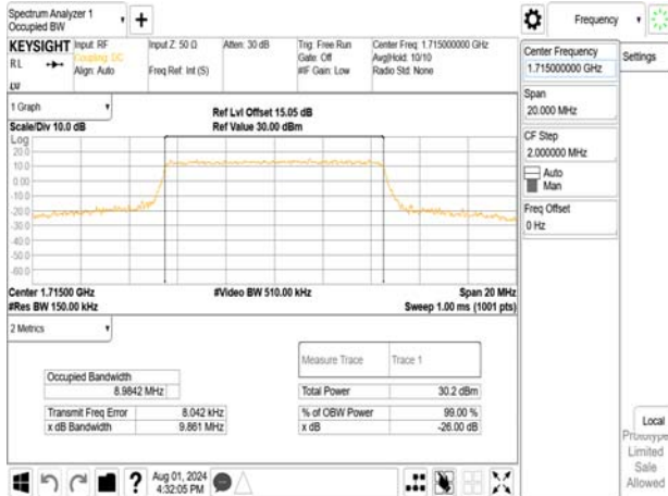
Band66_10MHz_64QAM_RB50_0_CH13222
