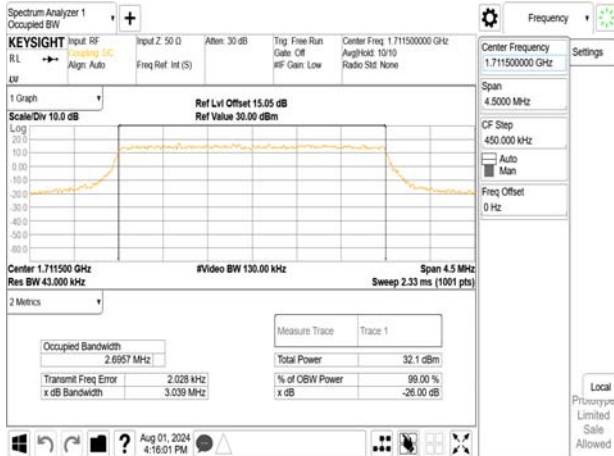
Band66_3MHz_QPSK_RB15_0_CH13222
