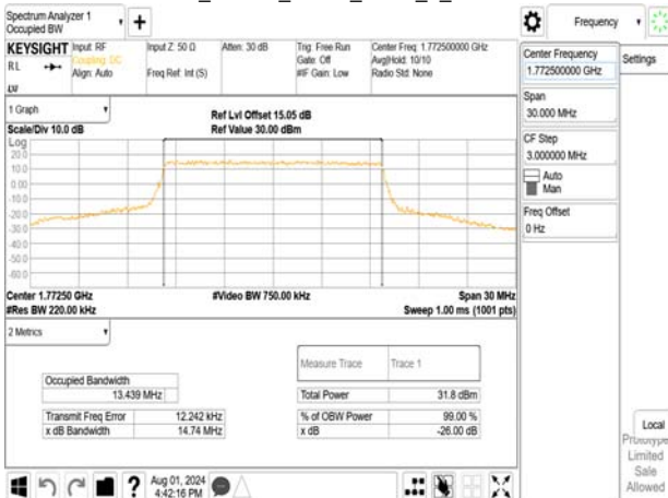
Band66_15MHz_QPSK_RB75_0_CH132597
