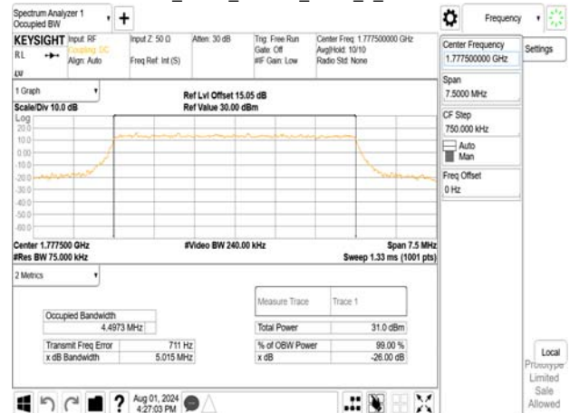
Band66_5MHz_16QAM_RB25_0_CH132647
