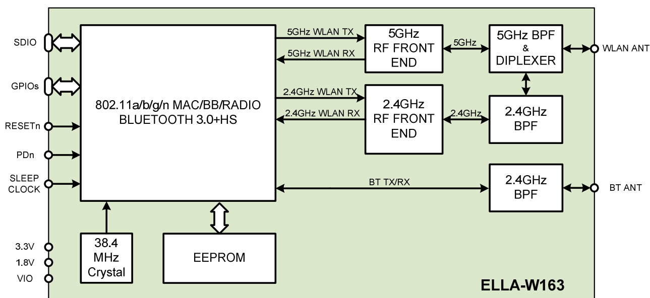
Figure 4: ELLA-W163 block diagram
