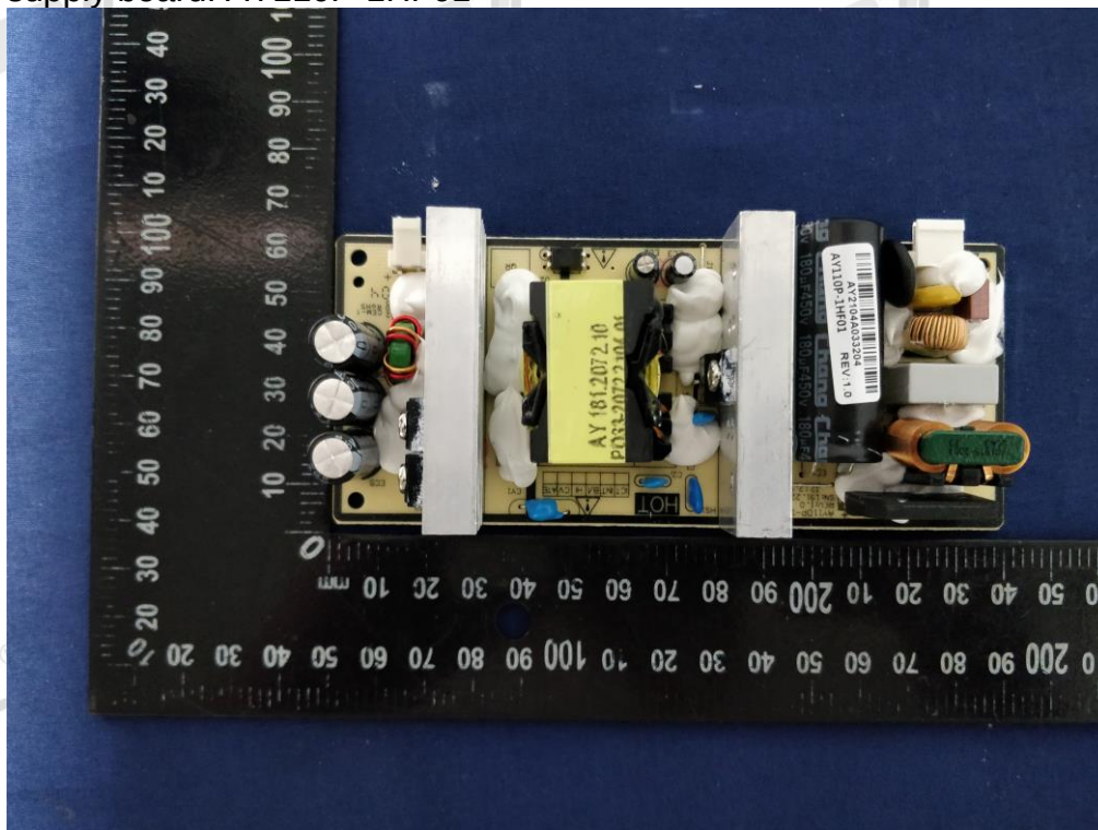
Power supply board: AY110P-1HF01
