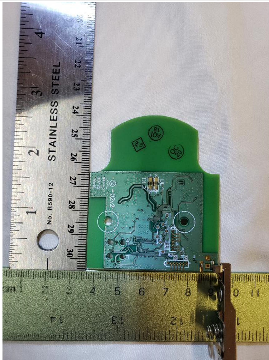
Figure 2. PCB – Back
