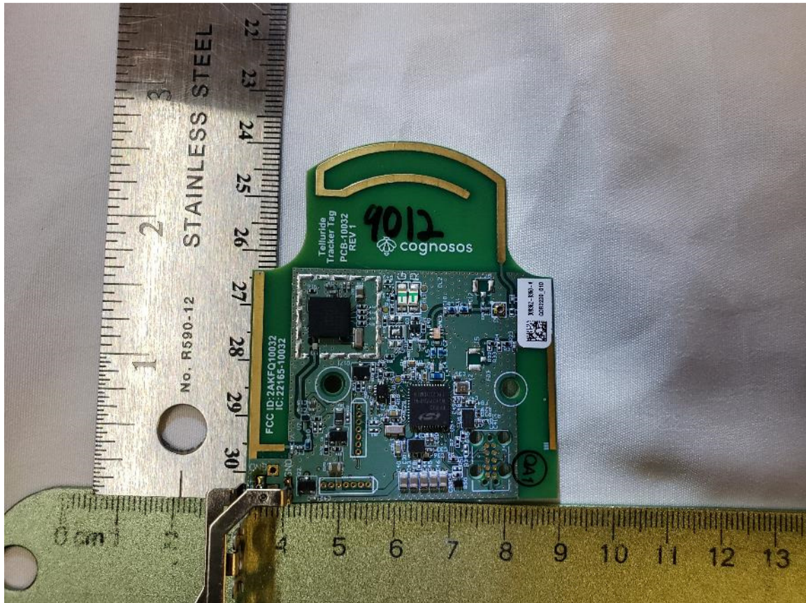
Figure 1. PCB – Front
