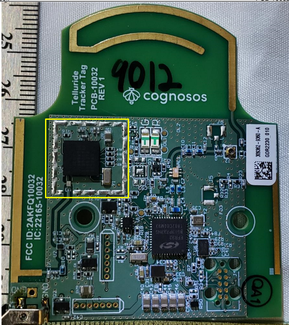
Figure 3. Radio Circuit
