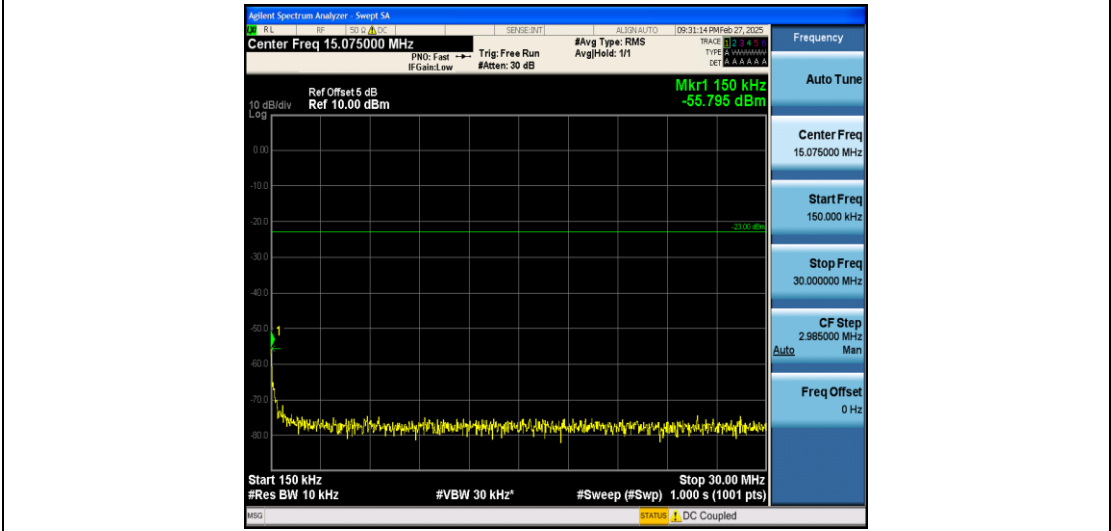
Band26_1.4MHz_QPSK_26697_1RB#0_0.15~30_0.15~30
