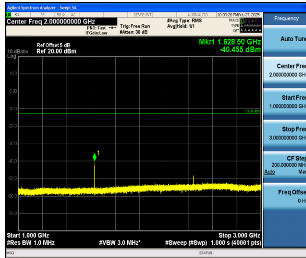
Band26_3MHz_QPSK_26705_1RB#0_1000~3000_1000~3000
