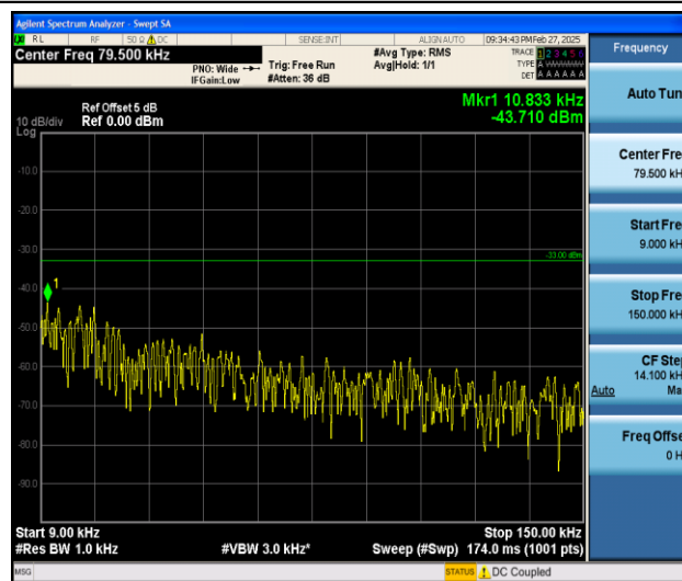
Band26_1.4MHz_QPSK_26783_1RB#0_0.009~0.15_0.009~0.15
