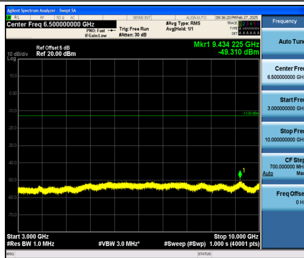
Band26_1.4MHz_16QAM_26783_1RB#0_3000~10000_3000~10000
