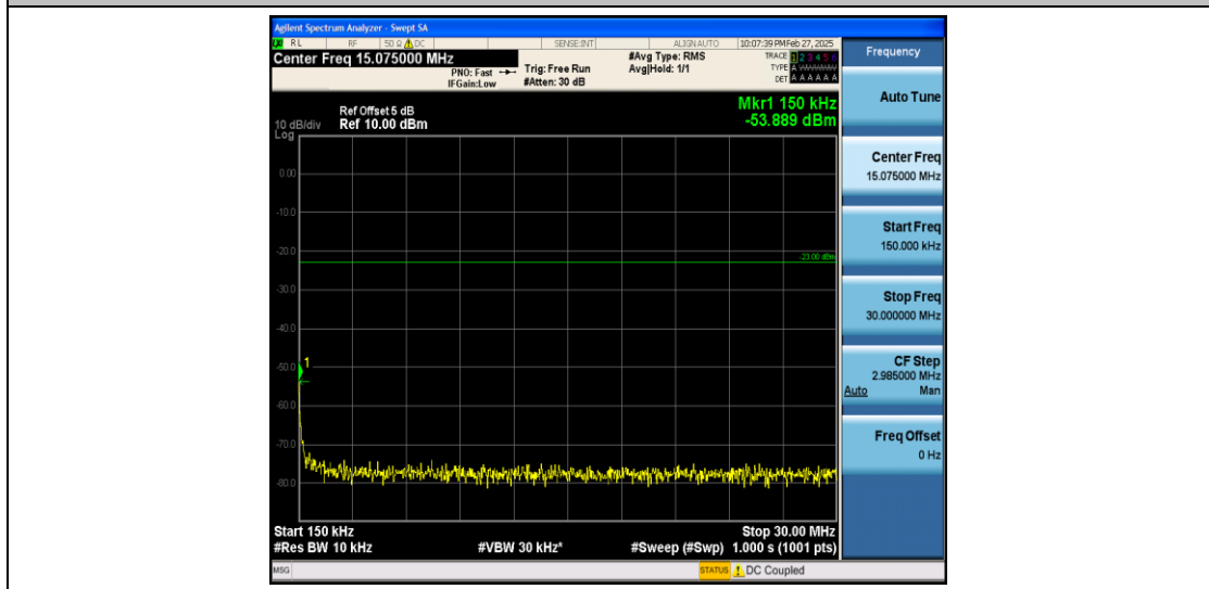
Band26_3MHz_16QAM_26775_1RB#0_0.15~30_0.15~30
