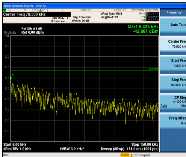
Band26_1.4MHz_QPSK_26740_1RB#0_0.009~0.15_0.009~0.15
