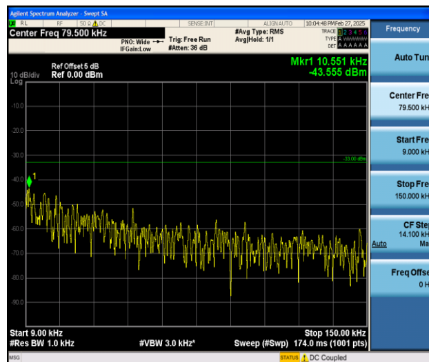
Band26_3MHz_QPSK_26740_1RB#0_0.009~0.15_0.009~0.15
