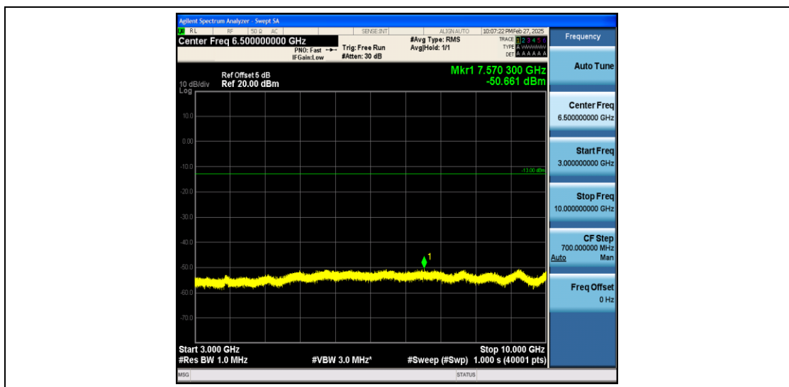
Band26_3MHz_QPSK_26775_1RB#0_3000~10000_3000~10000
