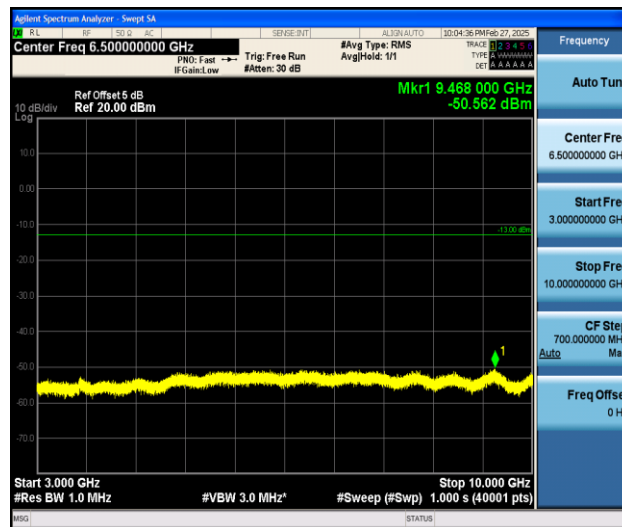
Band26_3MHz_16QAM_26705_1RB#0_3000~10000_3000~10000
