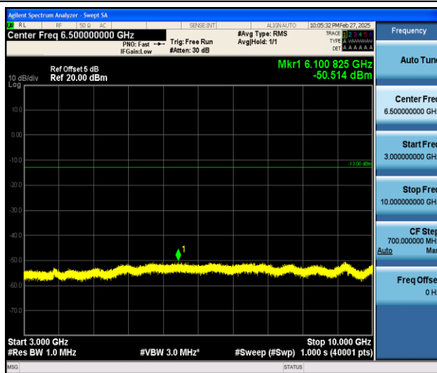
Band26_3MHz_QPSK_26740_1RB#0_3000~10000_3000~10000
