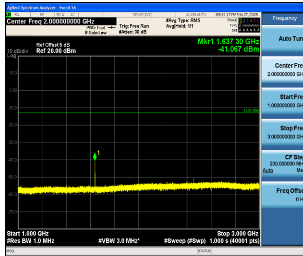
Band26_1.4MHz_16QAM_26740_1RB#0_1000~3000_1000~3000
