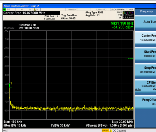
Band26_3MHz_QPSK_26740_1RB#0_0.15~30_0.15~30
