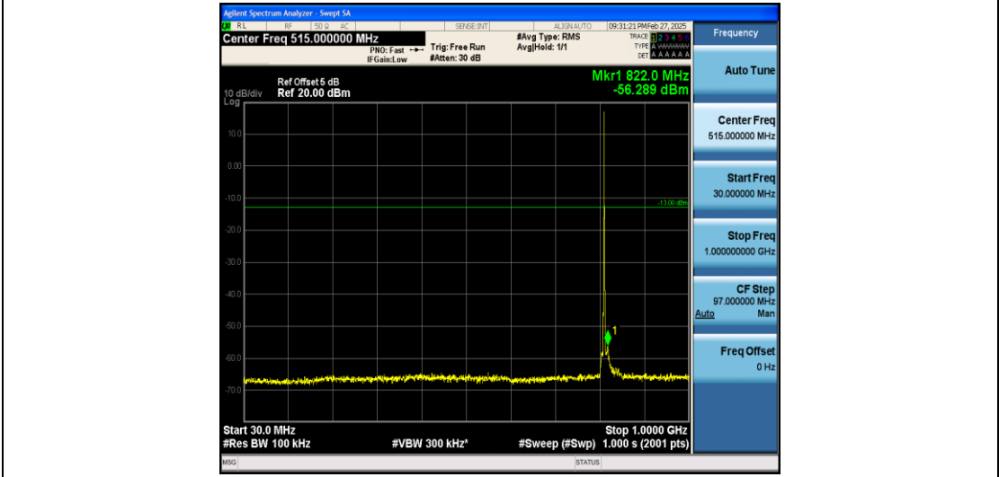
Band26_1.4MHz_QPSK_26697_1RB#0_30~1000_30~1000
