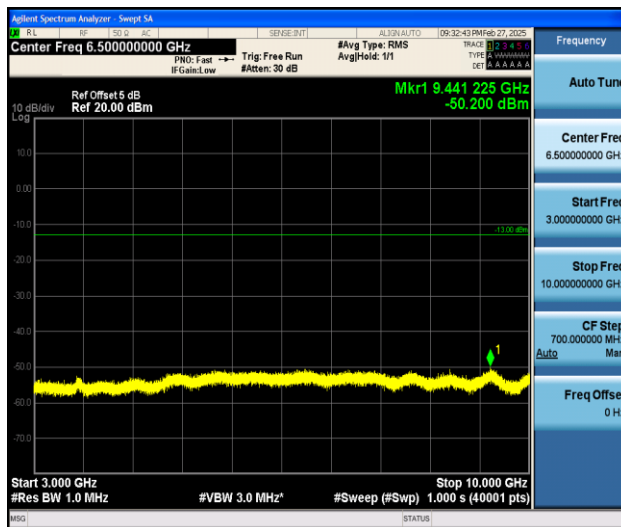
Band26_1.4MHz_16QAM_26697_1RB#0_3000~10000_3000~10000
