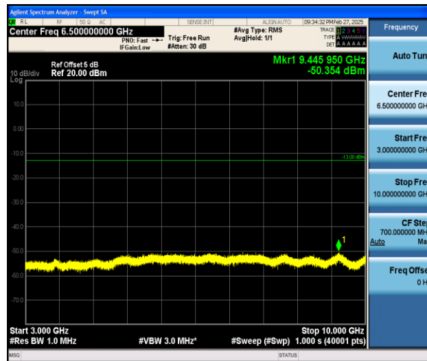
Band26_1.4MHz_16QAM_26740_1RB#0_3000~10000_3000~10000
