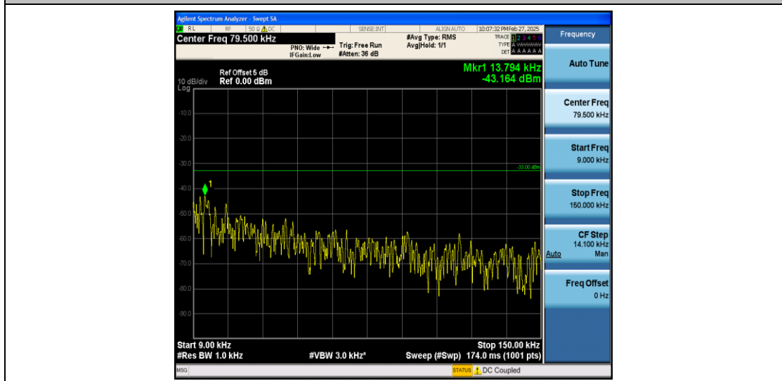
Band26_3MHz_16QAM_26775_1RB#0_0.009~0.15_0.009~0.15
