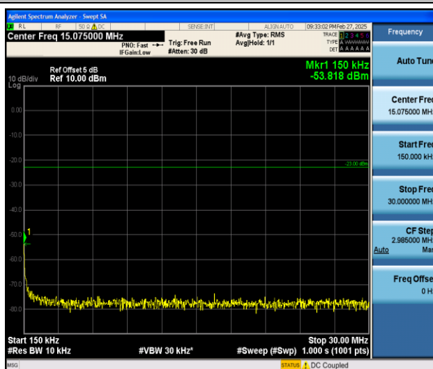
Band26_1.4MHz_QPSK_26740_1RB#0_0.15~30_0.15~30
