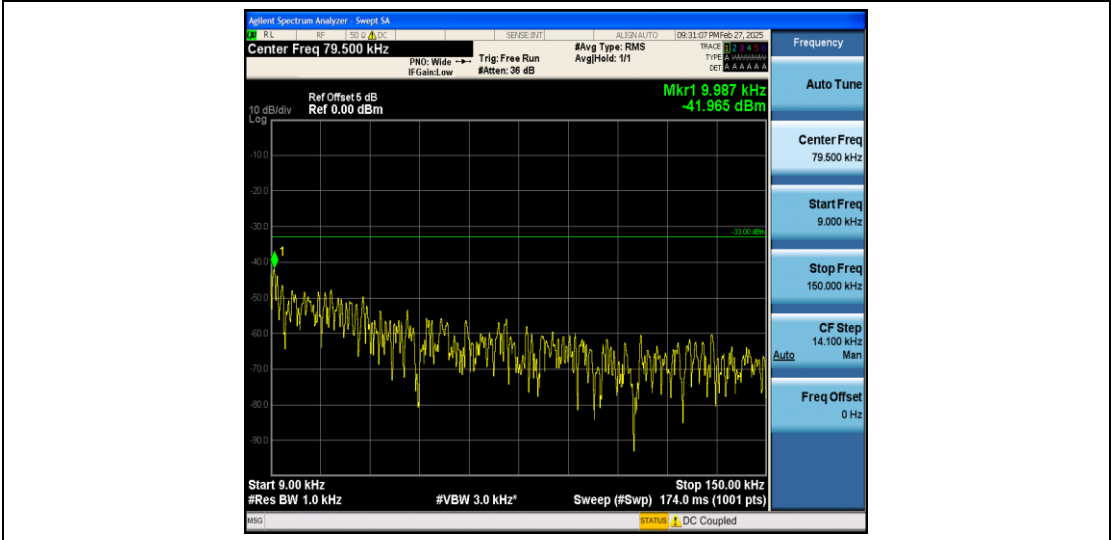
Band26_1.4MHz_QPSK_26697_1RB#0_0.009~0.15_0.009~0.15
