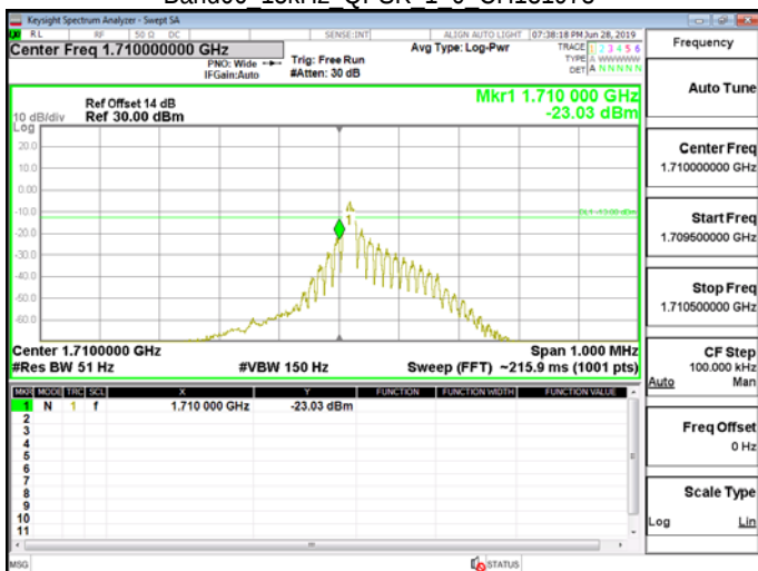
Band66 15kHz QPSK 1 0 CH131973
