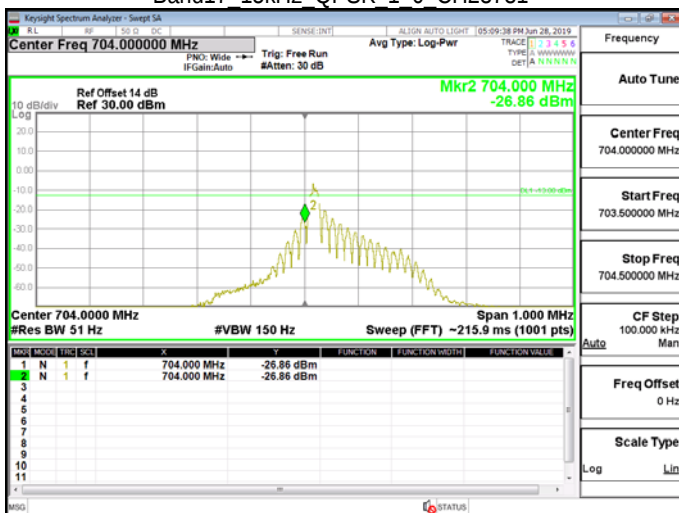
Band17 15kHz QPSK 1 0 CH23731
