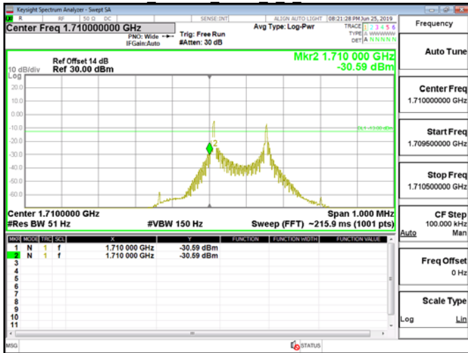
Band4 3.75kHz BPSK 1 47 CH20399
