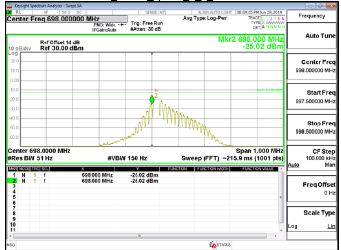
Band85 15kHz QPSK 1 11 CH134181
