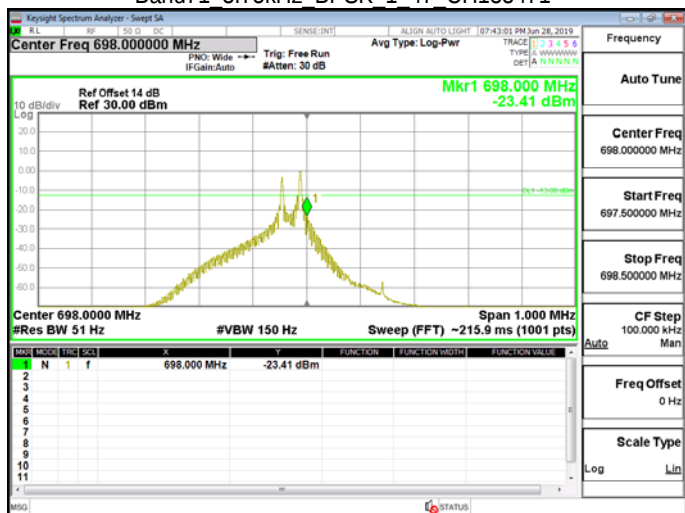
Band71 3.75kHz BPSK 1 47 CH133471
