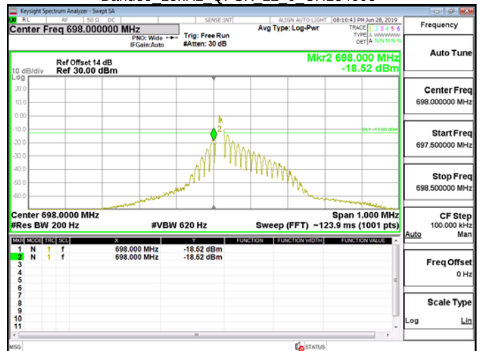
Band85 15kHz QPSK 12 0 CH134003
