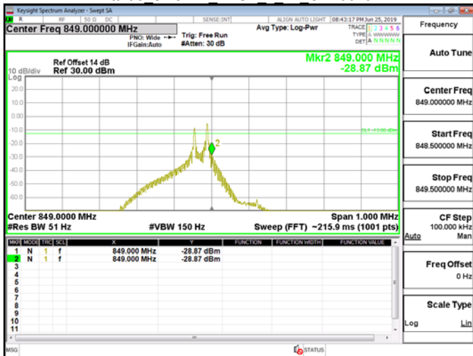
Band5 15kHz QPSK 1 0 CH20401
