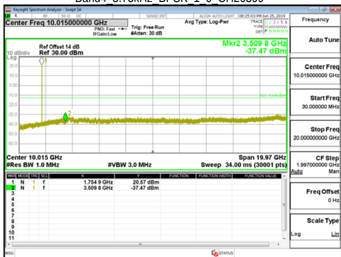
Band4 3.75kHz BPSK 1 0 CH20399
