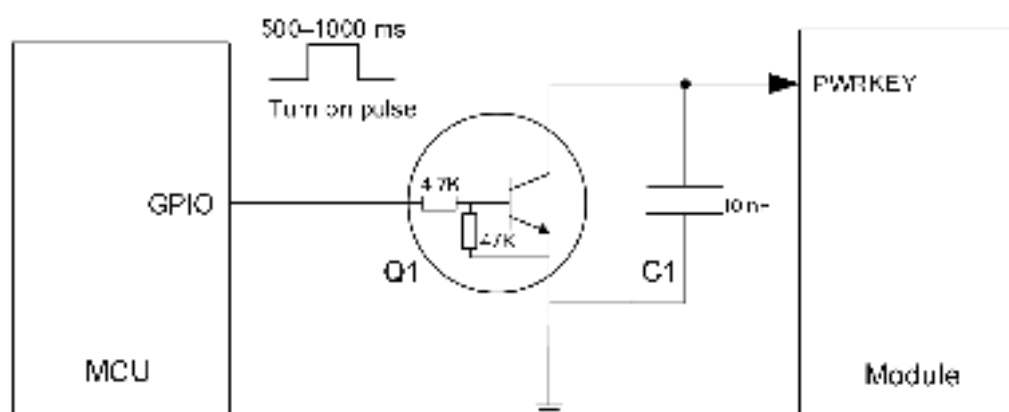
Figure 11: Turn On Module With a Driving Circuit
