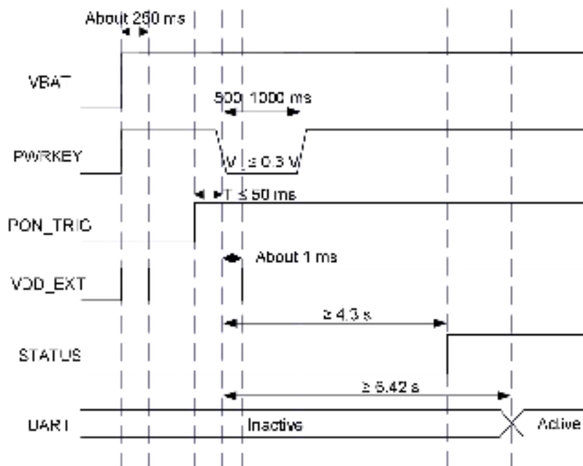
Figure 14: Power-up Timing (After VBAT is Stable for more than 250 ms)
