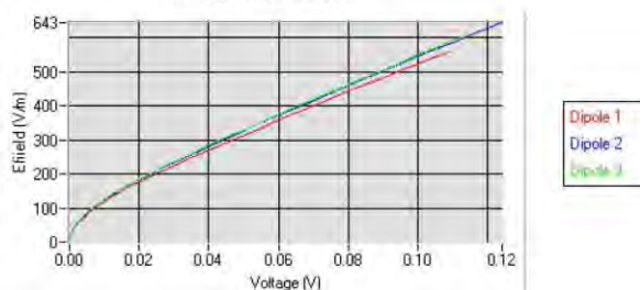
Calibration curves
