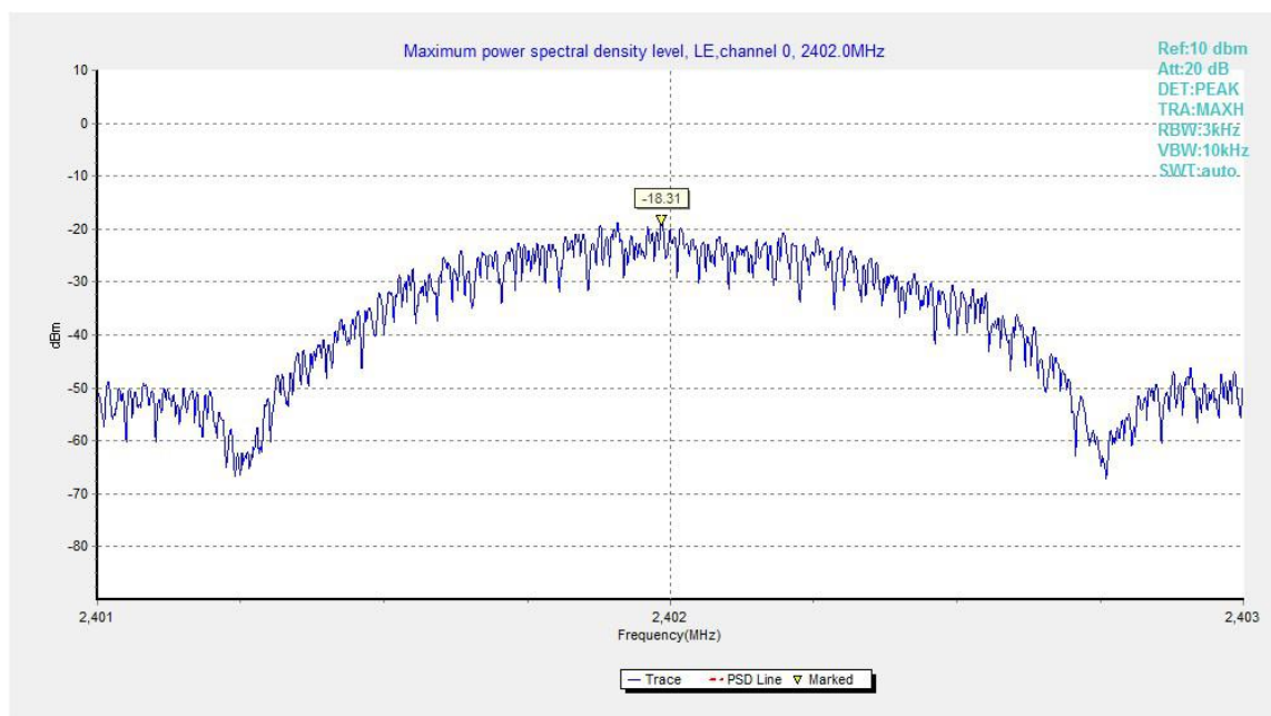
Fig.23. Maximum Power Spectral Density Level Function: GFSK, 2402 MHz
