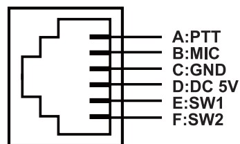
MIC JACK
