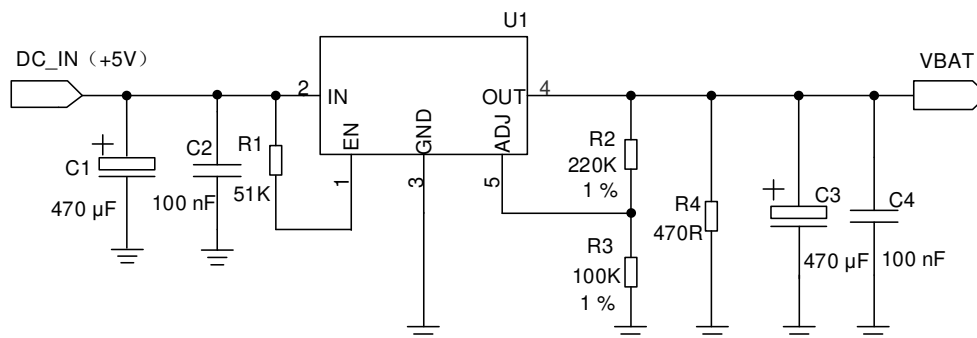
Figure 2: Reference Design of Power Supply
