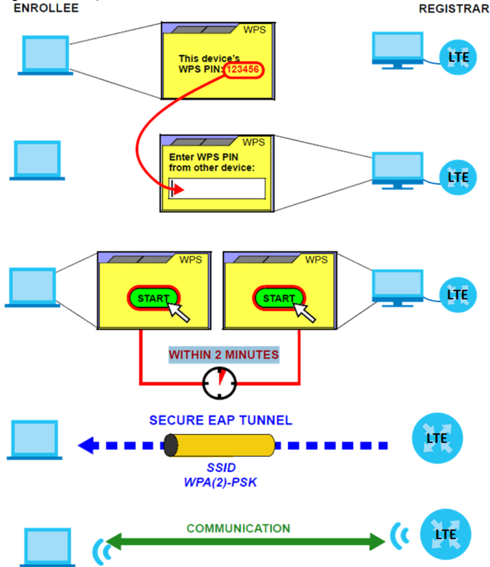
Figure 41 Example WPS Process: PIN Method
