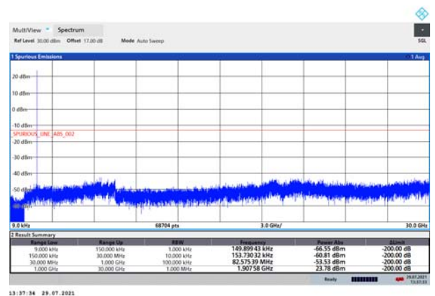
LTE Band 2 3MHz CH-High 9kHz~30GHz
