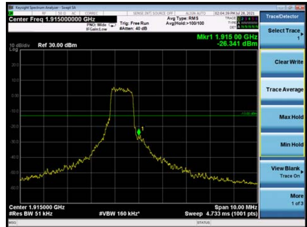
LTE Band 25 10MHz 16QAM 1RB CH-High
