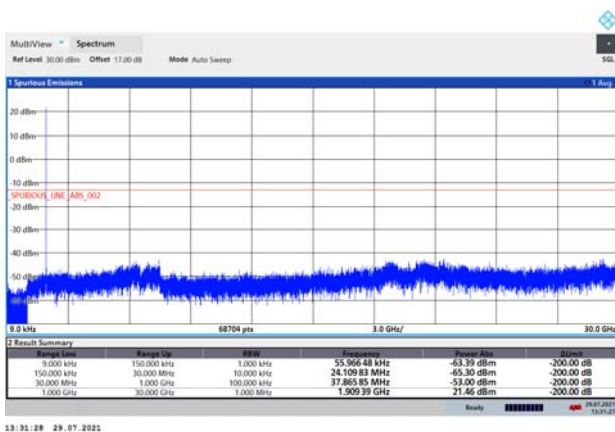
LTE Band 2 1.4MHz CH-High 9kHz~30GHz
