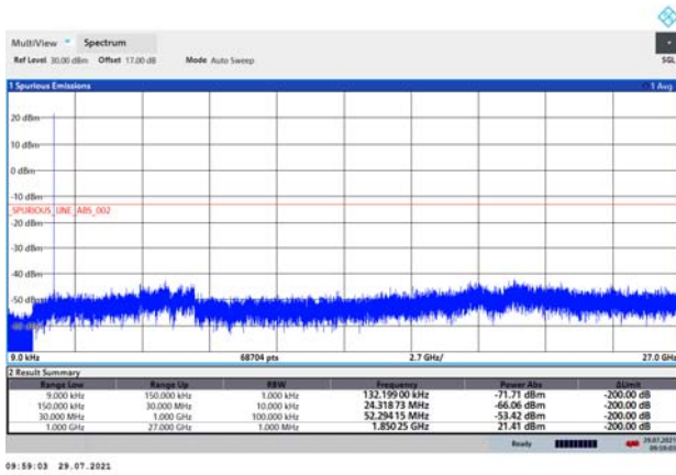
LTE Band 2 1.4MHz CH-Middle 9kHz~27GHz
