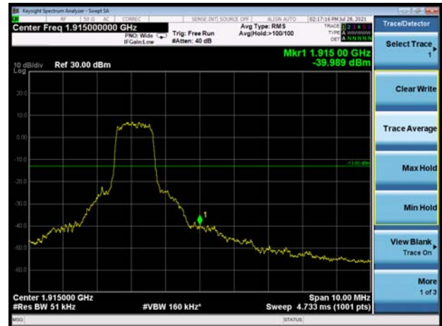
LTE Band 25 1.4MHz 16QAM 1RB CH-High
