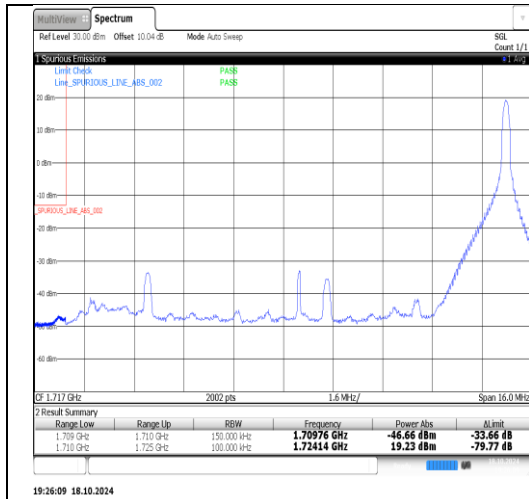
Band4-15MHz-16QAM-20325-75RB#0-PASS
