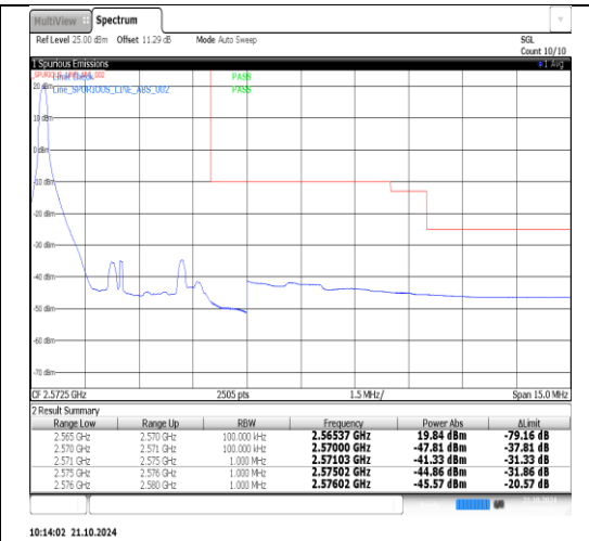
Band7-5MHz-16QAM-21425-1RB#24-PASS
