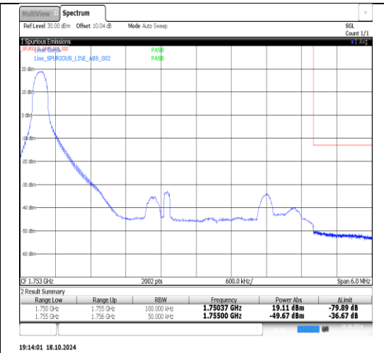
Band4-5MHz-16QAM-20375-1RB#24-PASS
