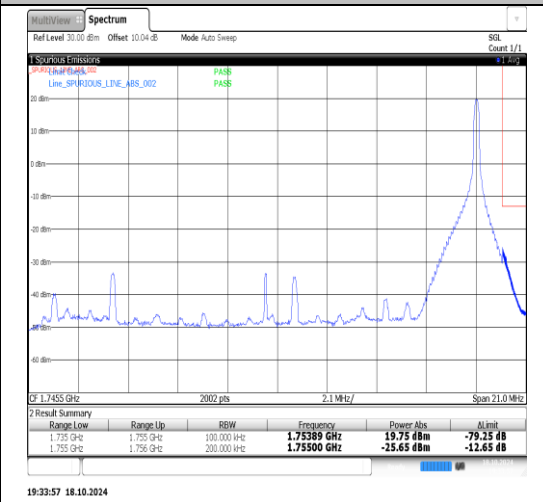
Band4-20MHz-16QAM-20050-100RB#0-PASS
