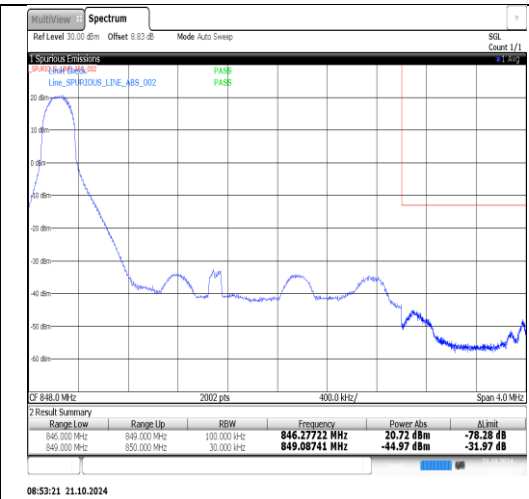
Band5-3MHz-16QAM-20635-1RB#14-PASS
