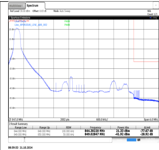
Band5-5MHz-QPSK-20625-1RB#24-PASS
