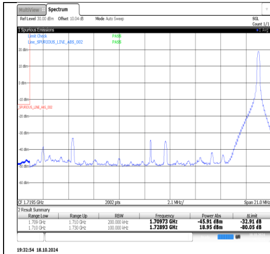
Band4-20MHz-QPSK-20300-100RB#0-PASS
