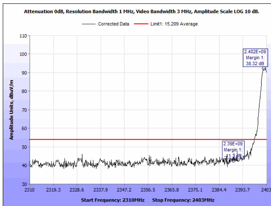
Plot 18. Radiated Band Edge, 2402 MHz, Peak on Average
