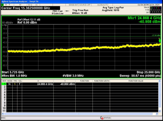
Spurious Emission:5725~25000.0 MHz IEEE 802.11ac_Channel 100_20MHz_Antenna 0
