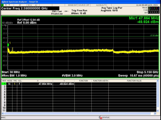
Spurious Emission:30.0~5150 MHz IEEE 802.11ac_Channel 64_20MHz_Antenna 0
