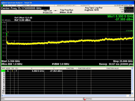
Spurious Emission:5350~25000.0 MHz IEEE 802.11ac_Channel 56_20MHz_Antenna 0
