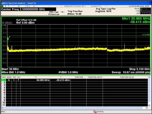
Spurious Emission:30.0~5150 MHz IEEE 802.11ac_Channel 56_20MHz_Antenna 0
