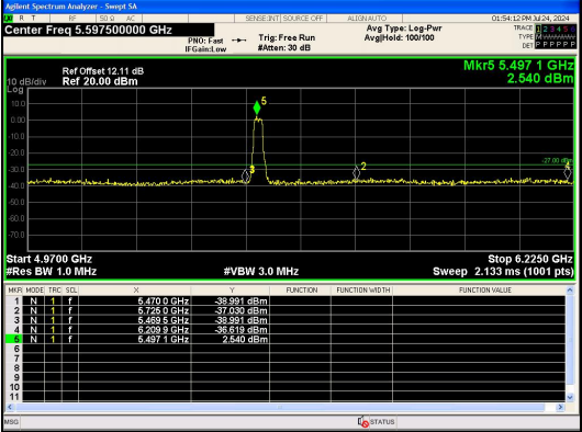
Out Of Band Emission IEEE 802.11ac_Channel 100_20MHz_Antenna 0
