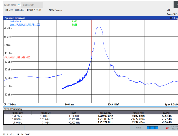
Band4-1.4MHz-QPSK-19957-6RB#0
