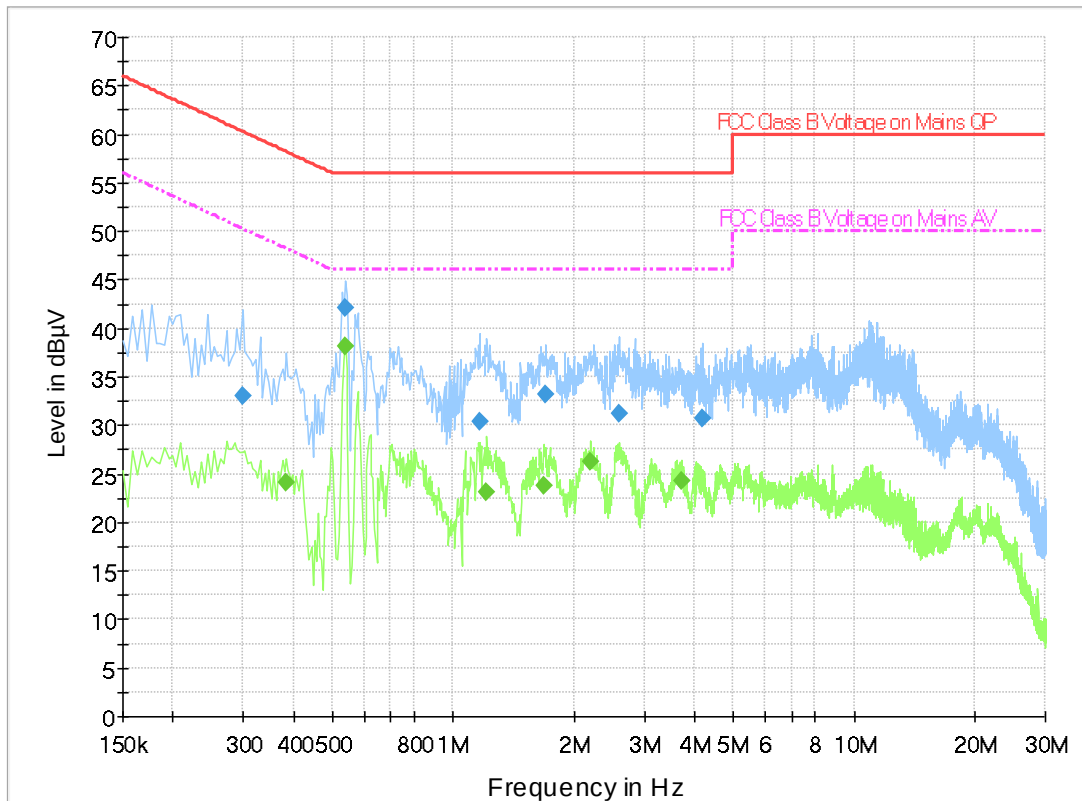
Fig.B.7.2 AC Powerline Conducted Emission-Idle
