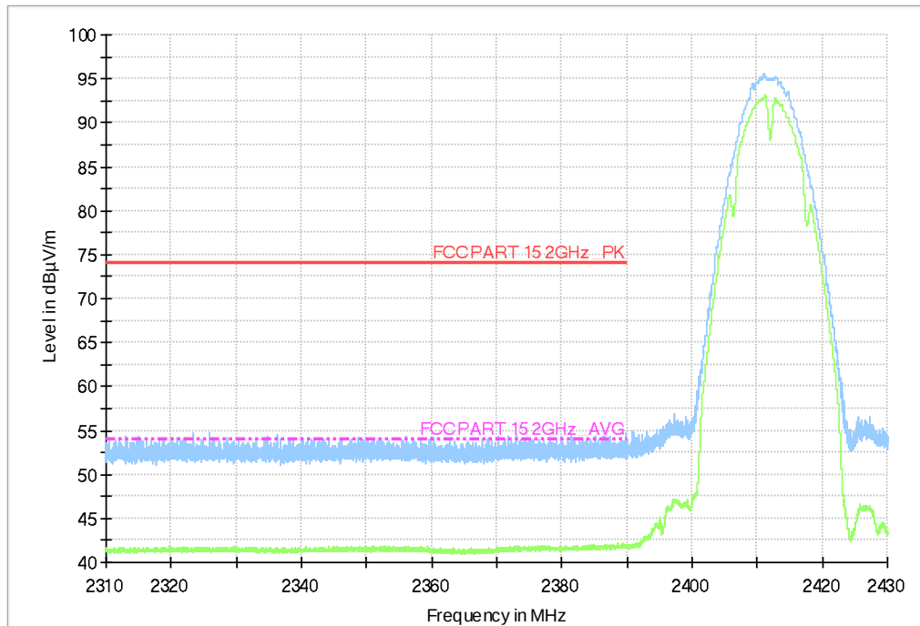
Fig.B.6.2.1 Transmitter Spurious Emission - Radiated (Power): 802.11b, ch1, 2.31 GHz – 2.43GHz
