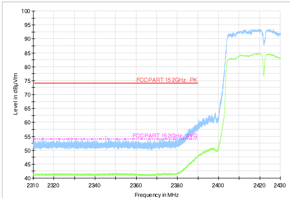
Fig.B.6.2.7 Transmitter Spurious Emission - Radiated (Power): 802.11n-HT40, ch3, 2.31 GHz - 2.43GHz
