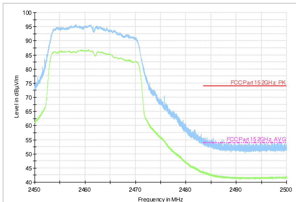
Fig.B.6.2.6 Transmitter Spurious Emission - Radiated (Power): 802.11n-HT20, ch11, 2.45 GHz - 2.50GHz
