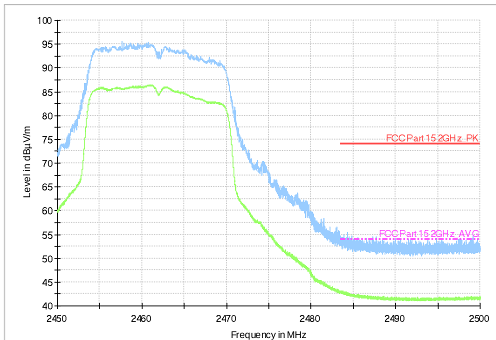
Fig.B.6.2.4 Transmitter Spurious Emission - Radiated (Power): 802.11g, ch11, 2.45 GHz - 2.50GHz
