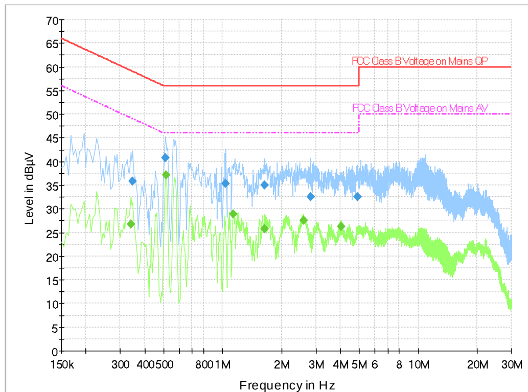
Fig.B.7.1 AC Powerline Conducted Emission-Traffic
