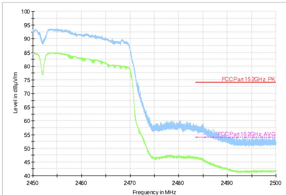
Fig.B.6.2.8 Transmitter Spurious Emission - Radiated (Power): 802.11n-HT40, ch11, 2.45 GHz - 2.50GHz
