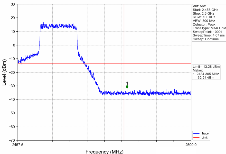
10MHz BW_HCH_2467.5MHz_Ant1_NTNV
