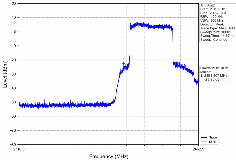
40MHz BW_LCH_2422.5MHz_Ant2_NTNV
