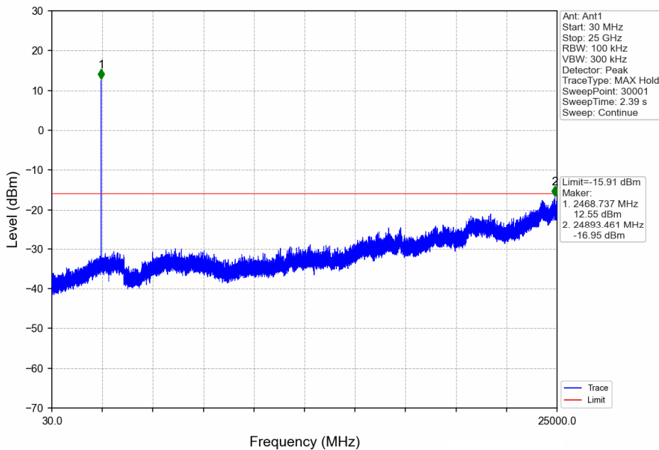
3MHz BW_HCH_2468.5MHz_Ant1_NTNV
