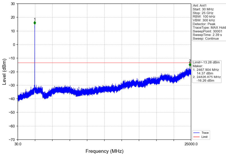
10MHz BW_HCH_2467.5MHz_Ant1_NTNV
