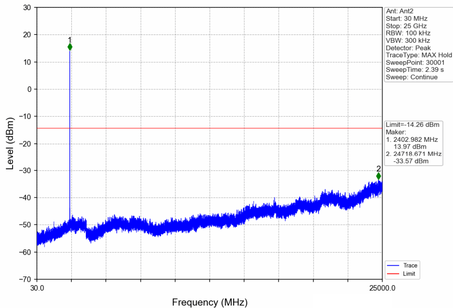
1.4MHz BW_LCH_2403.5MHz_Ant2_NTNV
