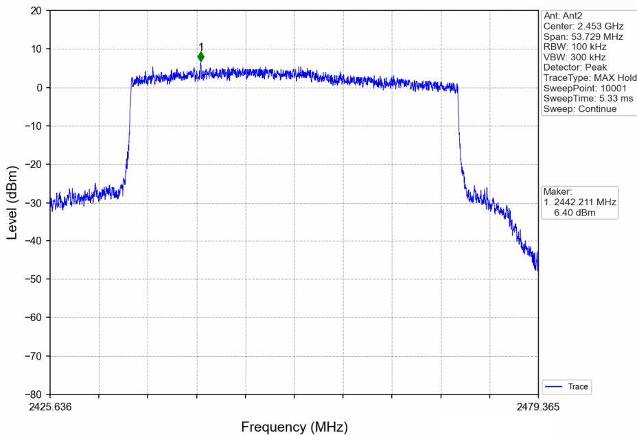
40MHz BW_HCH_2452.5MHz_Ant2_NTNV
