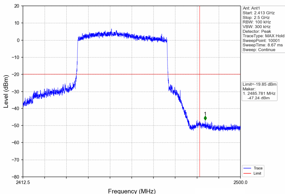
40MHz BW_HCH_2452.5MHz_Ant1_NTNV
