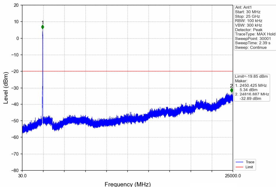
40MHz BW_HCH_2452.5MHz_Ant1_NTNV
