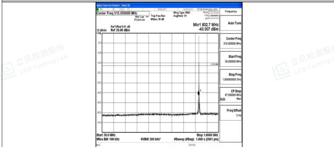
Band5-1.4MHz-16QAM-20525-1RB#0-30~1000-PASS
