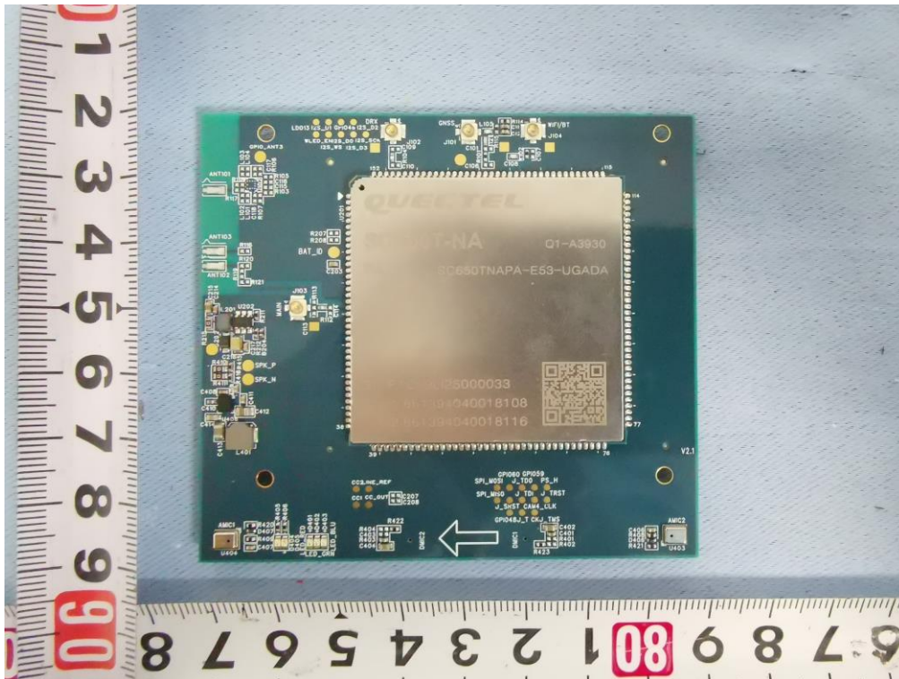
Test PCB board Photo-- SC650T-NA
