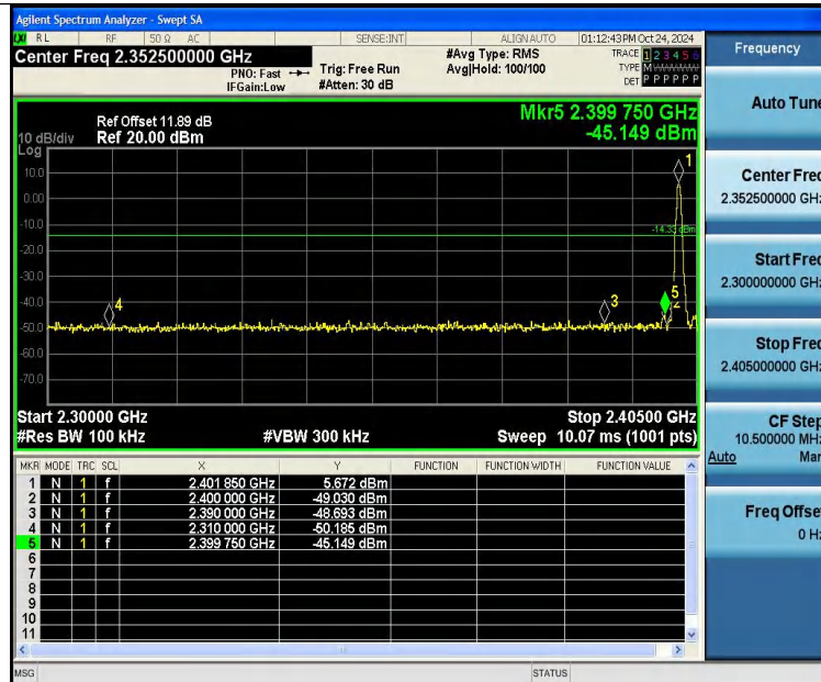
DH5-Ant1-2402-PASS
