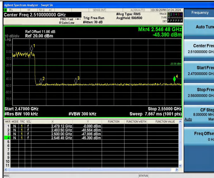
2DH5-Ant1-Hop_2480-PASS
