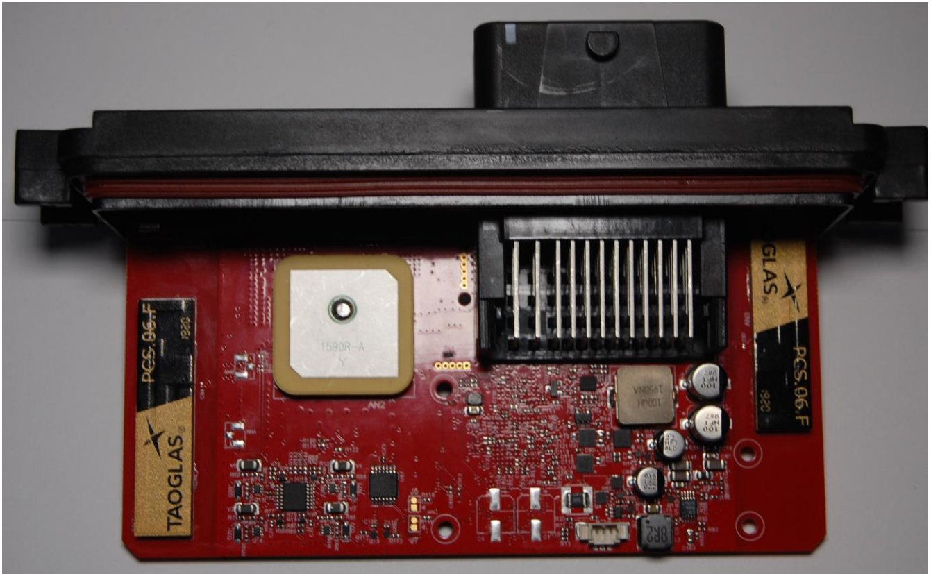
Assembled Unit – Top Side (Battery Removed)
