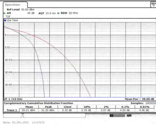
Band4-10MHz-QPSK-20175-1RB#0
