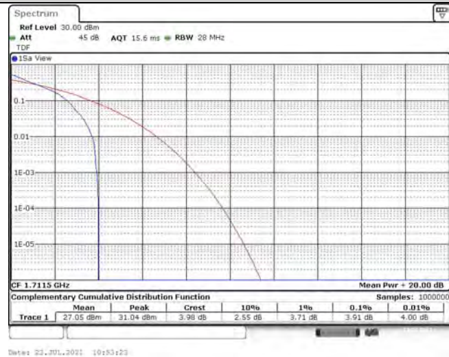
Band4-3MHz-QPSK-19965-15RB#0
