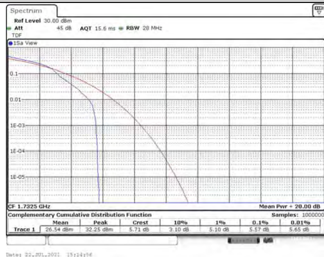
Band4-3MHz-16QAM-20175-15RB#0
