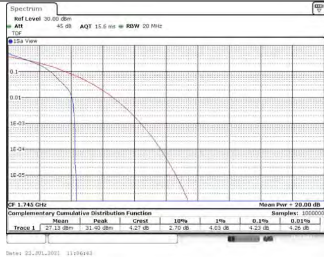
Band4-5MHz-QPSK-20300-25RB#0
