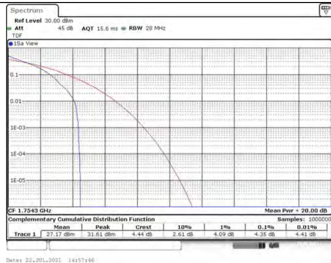
Band4-1.4MHz-QPSK-20393-6RB#0
