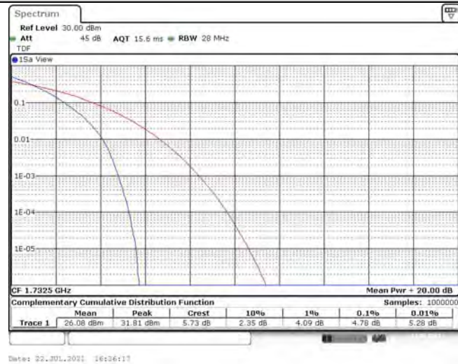
Band4-20MHz-QPSK-20300-1RB#0
