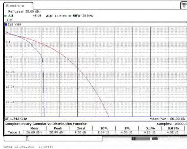
Band4-15MHz-QPSK-20300-75RB#0
