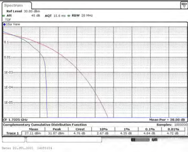
Band4-1.4MHz-QPSK-20175-1RB#0
