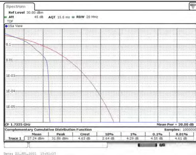
Band4-10MHz-QPSK-20175-50RB#0
