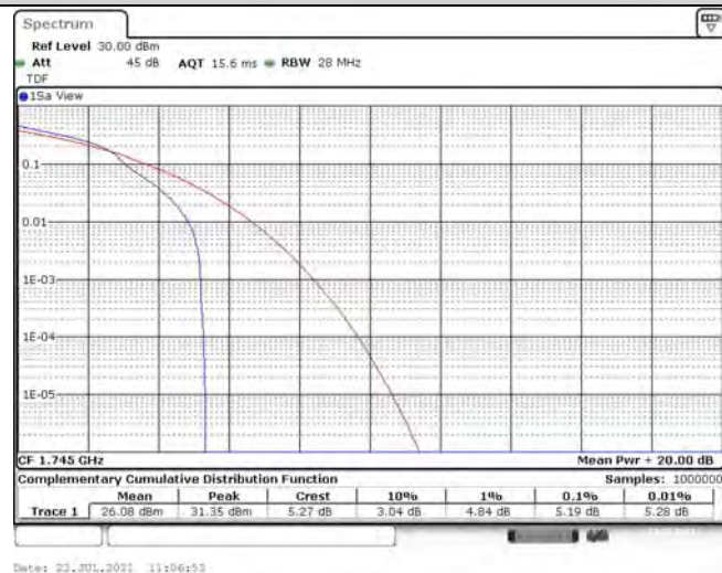
Band4-5MHz-16QAM-20300-25RB#0
