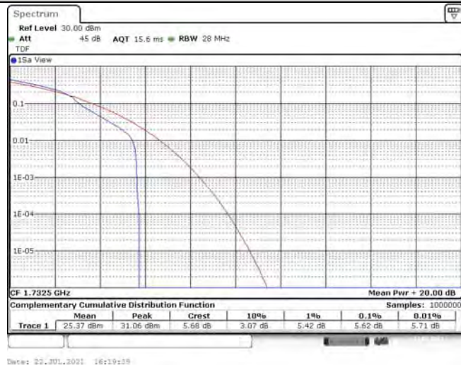
Band4-15MHz-16QAM-20175-75RB#0
