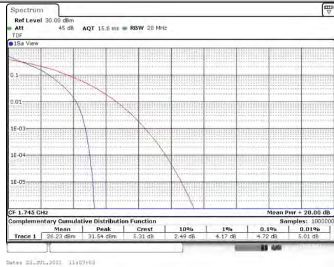
Band4-5MHz-QPSK-20375-1RB#0
