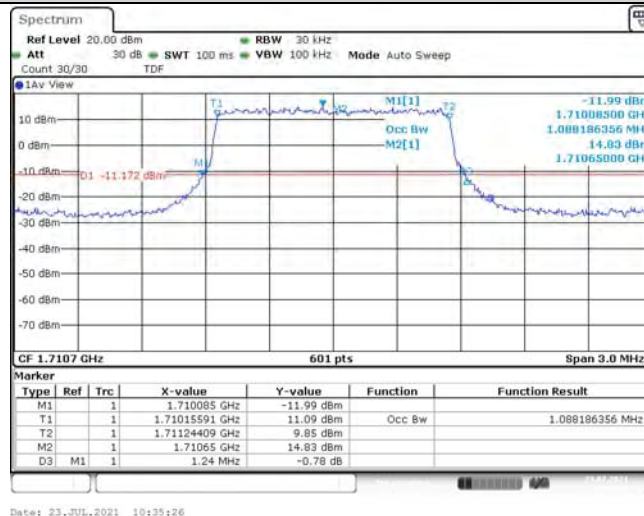
Band4-1.4MHz-QPSK-20175-6RB#0-1.088
