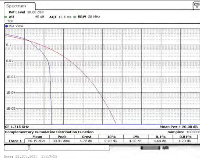
Band4-10MHz-16QAM-20000-50RB#0
