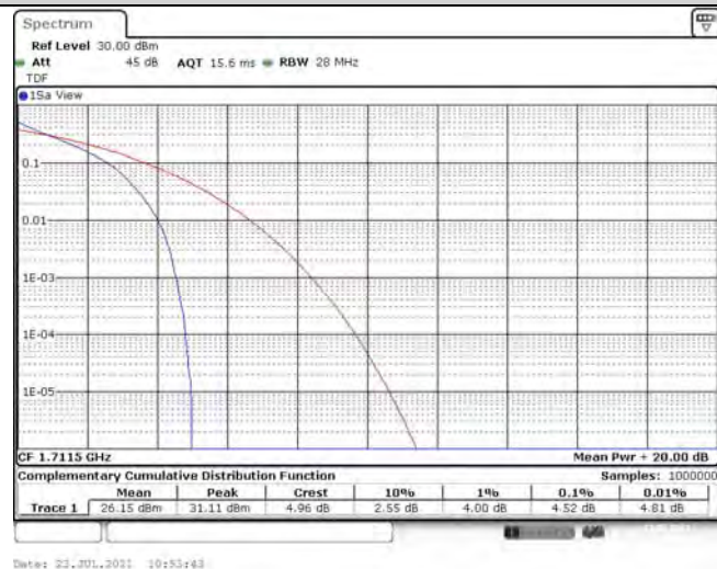
Band4-3MHz-QPSK-20175-1RB#0
