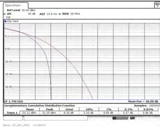
Band4-15MHz-16QAM-20325-1RB#0
