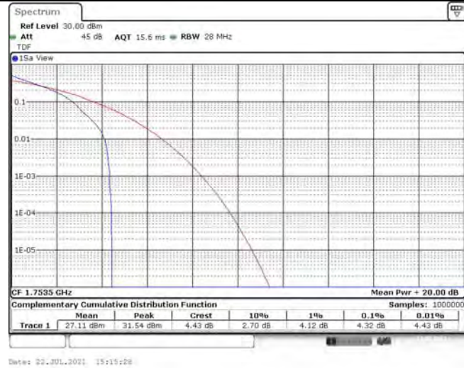
Band4-3MHz-QPSK-20385-15RB#0
