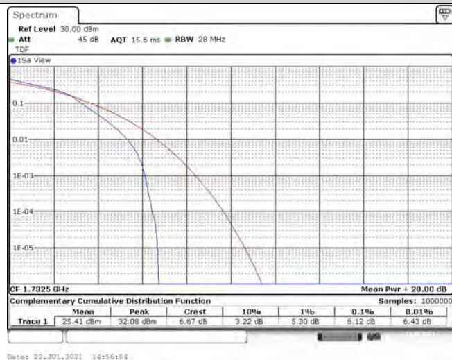
Band4-1.4MHz-16QAM-20300-1RB#0
