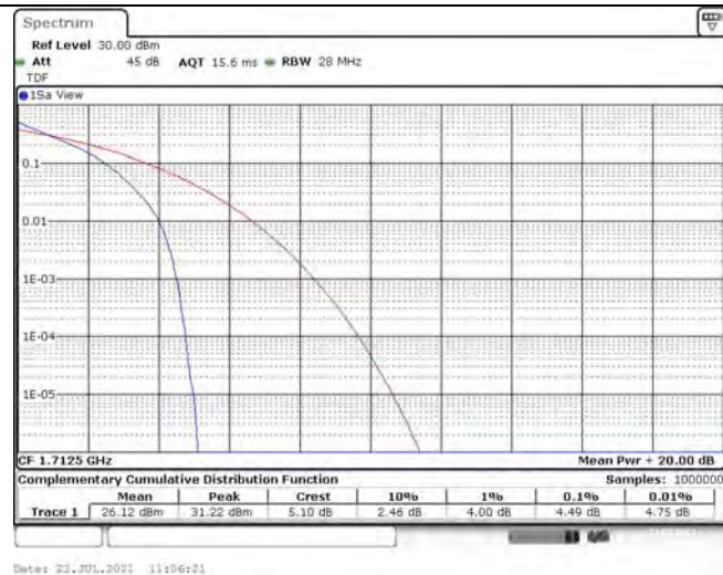
Band4-5MHz-QPSK-20175-1RB#0
