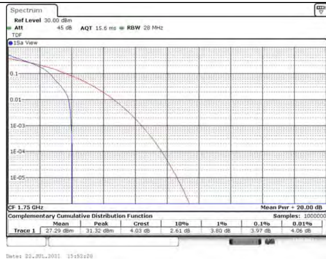
Band4-10MHz-QPSK-20350-50RB#0
