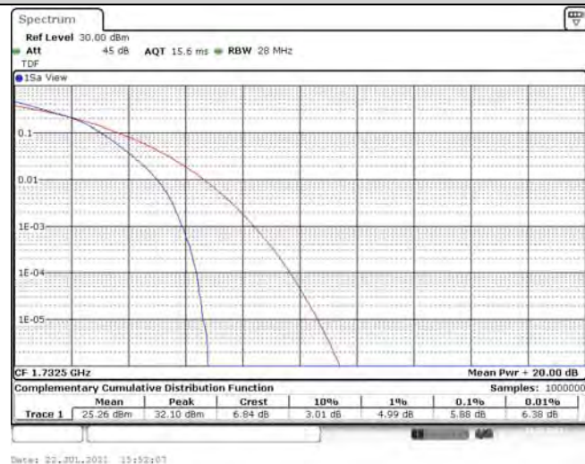
Band4-10MHz-16QAM-20300-1RB#0
