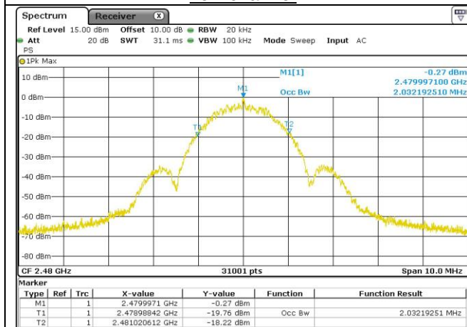
High channel
