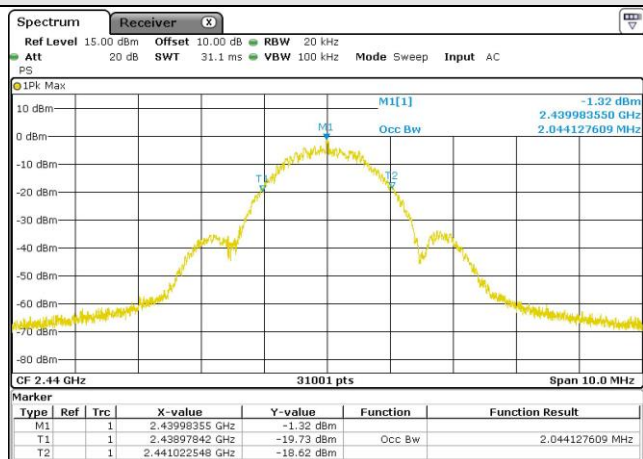
Mid channel
