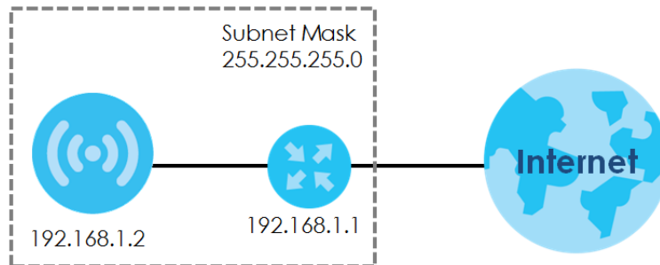
Figure 41 IP Setup
