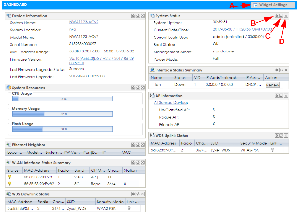
Figure 27 Dashboard
