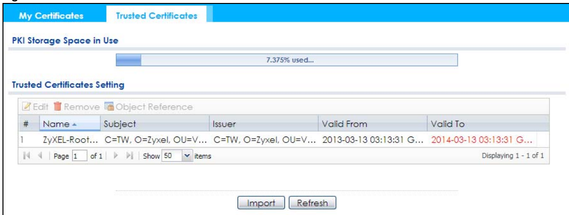
Figure 100 Trusted Certificates
