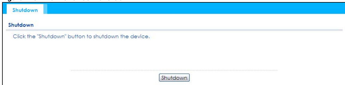
Figure 128 Maintenance > Shutdown
