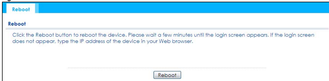
Figure 127 Maintenance > Reboot
