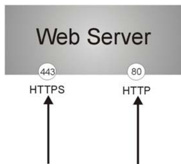
Figure 95 HTTP/HTTPS Implementation
