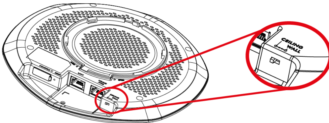
Figure 125 WAC6103D-I Physical Antenna Switch
