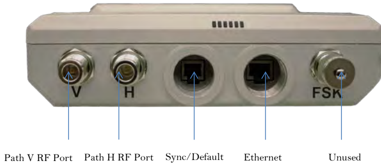
Figure 5 AP interfaces - 5 GHz original layout
