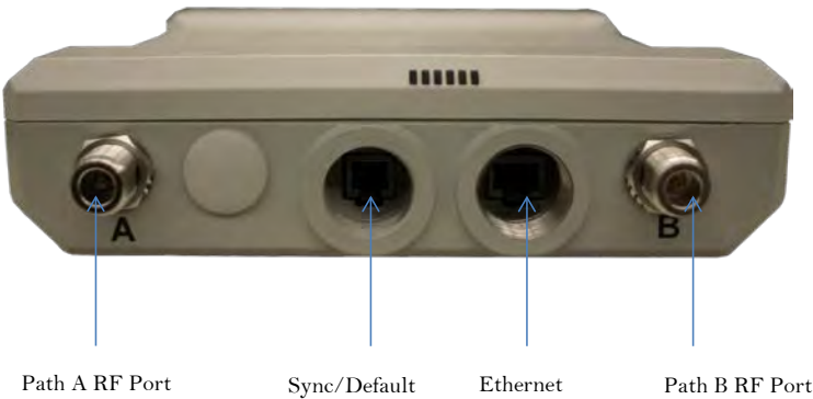
Figure 4 AP interfaces – 2.4 GHz, 3.5 GHz, 3.6GHz, 5 GHz
