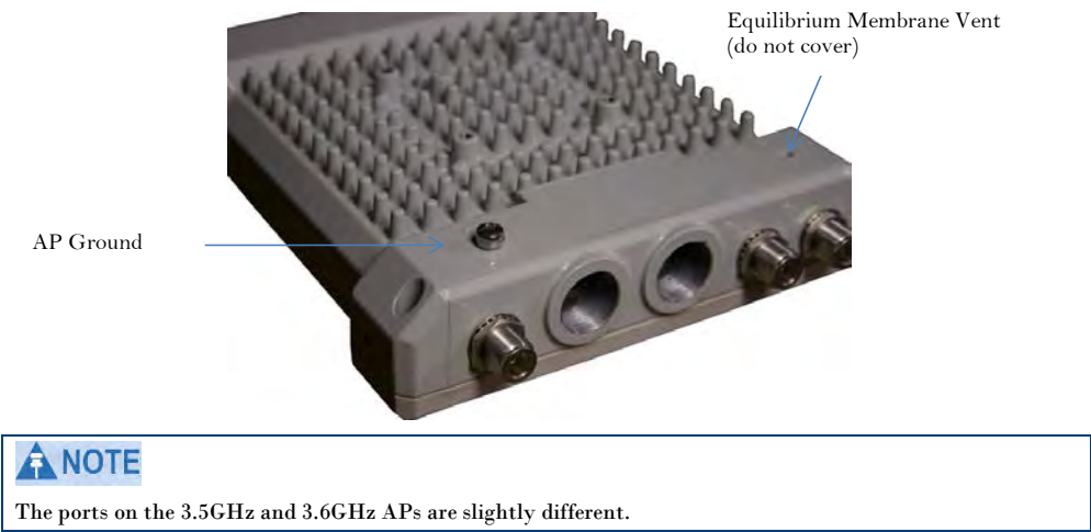
Figure 6 AP ground and equilibrium membrane vent
