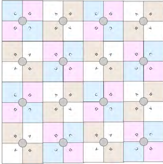
Figure 18 Example layout of 16 Access Point sectors (ABCD), 90 degree sectors
