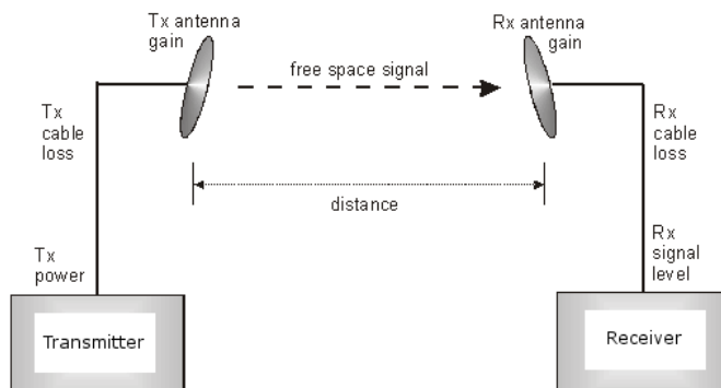
Figure 17 Determinants in Rx signal level
