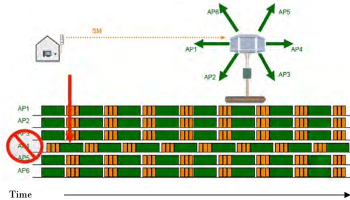
Figure 28 One unsynchronized AP in cluster resulting in self-interference
