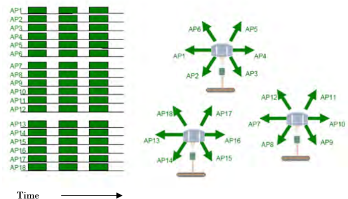
Figure 29 GPS timing throughout the network
