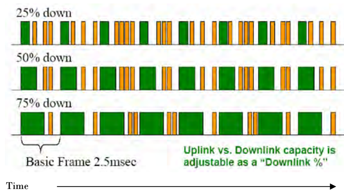
Figure 15 TDD Frame Division
