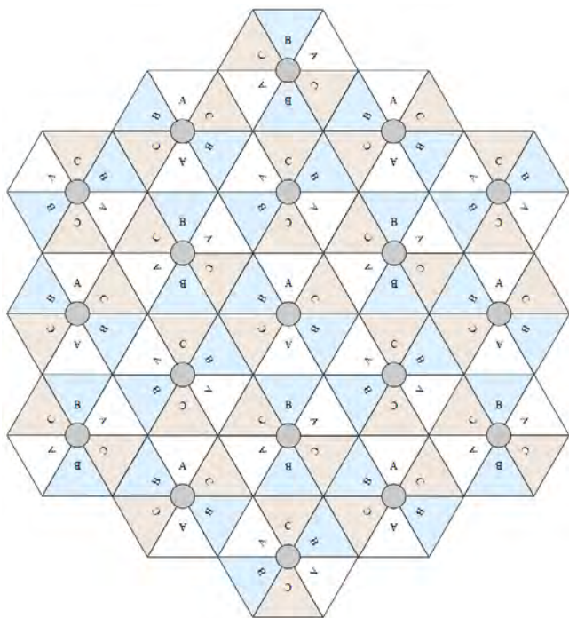
Figure 19 Example layout of 16 Access Point sectors (ABC), 60 degree sectors
