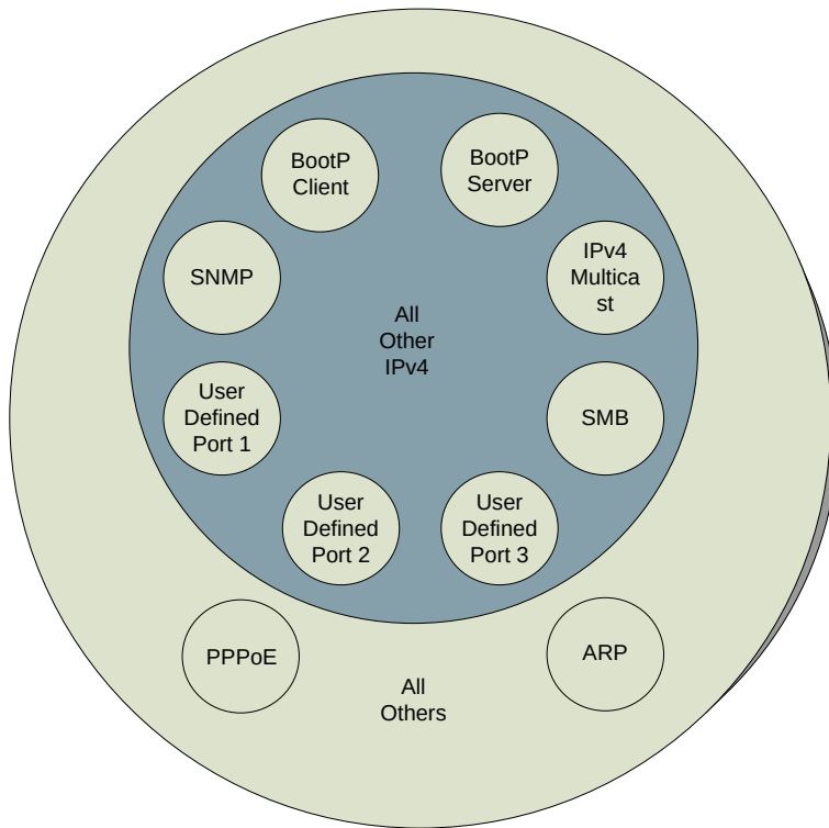
Figure 32 Categorical protocol filtering
