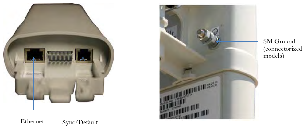
Figure 10 SM interfaces
