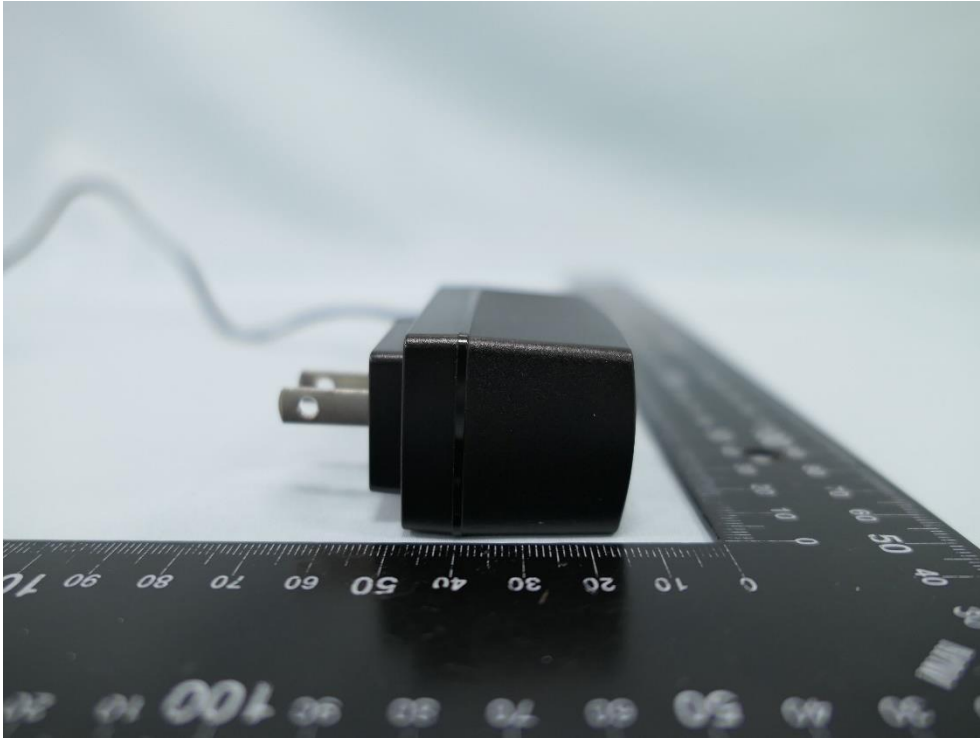
(14) EUT Photo (Brand: tp-link, MN: T120100-2B1)
