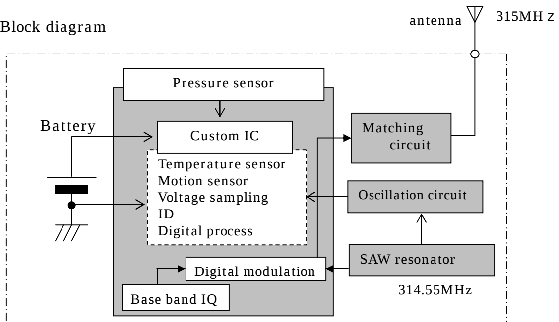
Fig 6, Block diagram of transmitter
