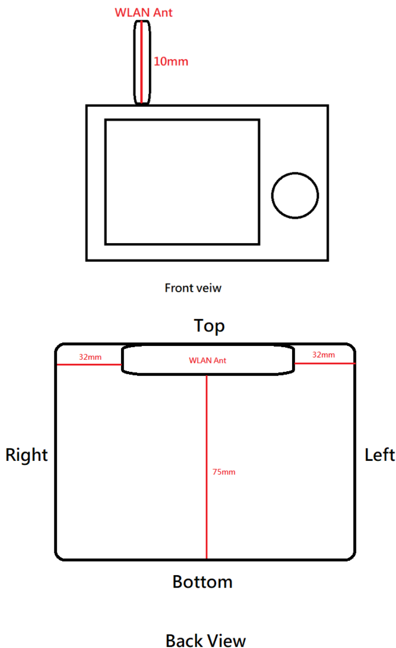
Photograph 9. Antenna position of EUT
