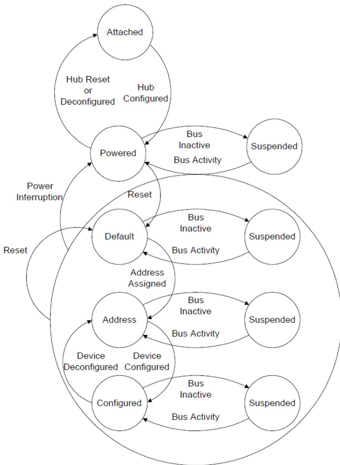
Figure 6-1. Device State Diagram
