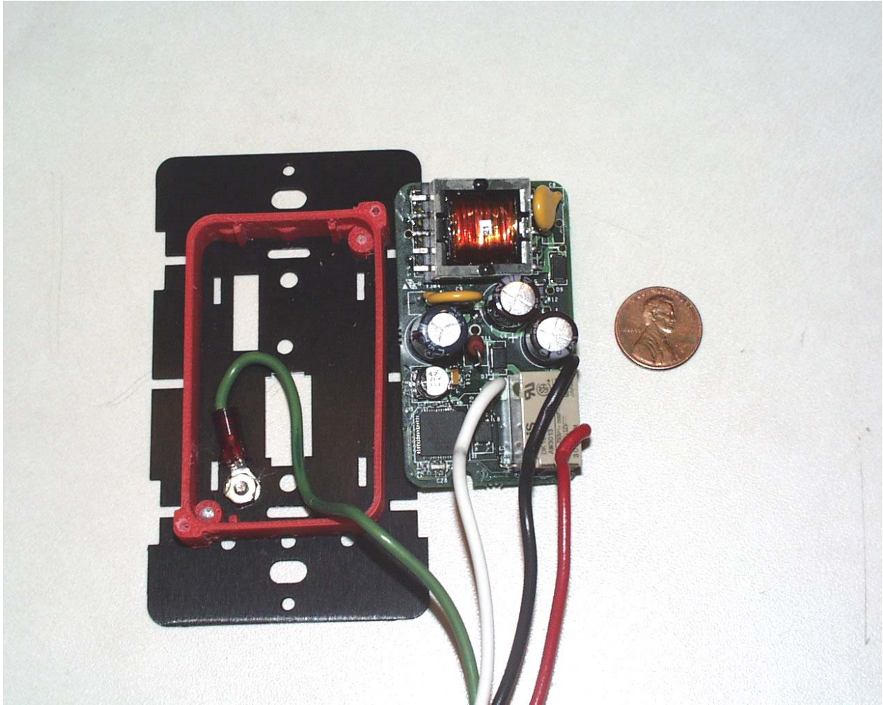
Photograph 7 - View of the Component Side of the Host Card
