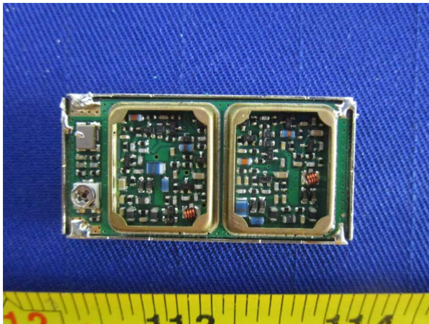
EUT – Board Uncover View
