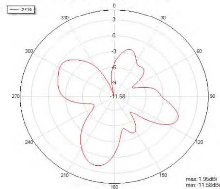
Theta=90 freq=2416MHz
