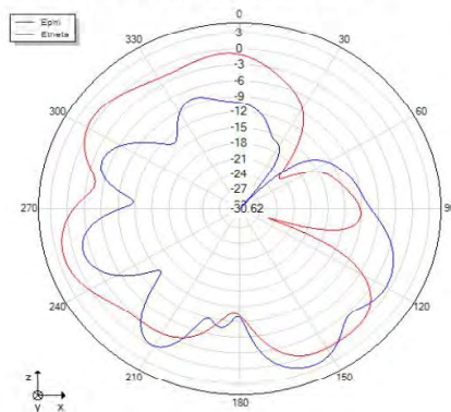
Phi=0 freq=2416MHz
