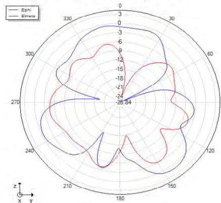
Phi=90 freq=2428MHz
