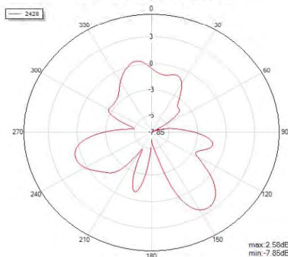
Phi=90 freq=2428MHz
