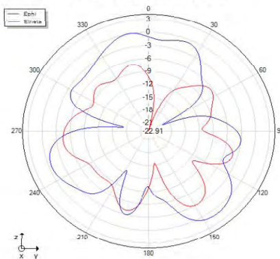
Phi=90 freq=2416MHz
