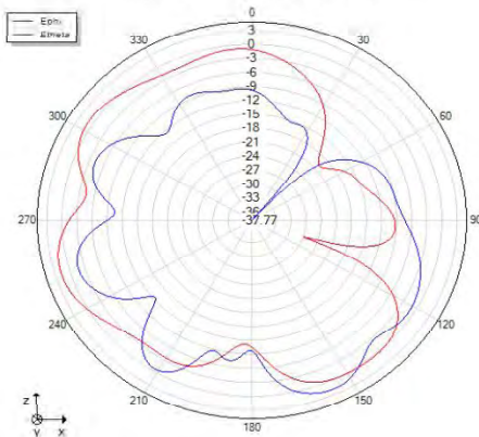
Phi=0 freq=2428MHz
