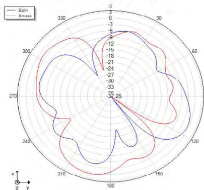
Theta=90 freq=2416MHz
