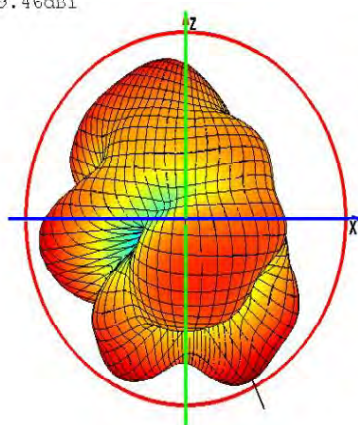
Phi=0 freq=2416MHz
