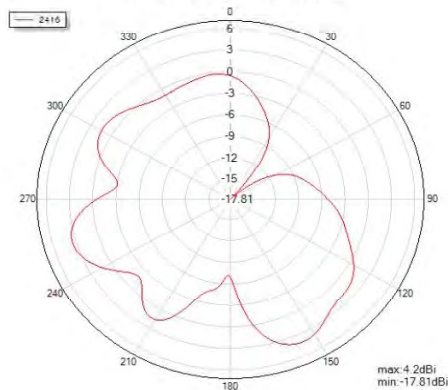
Phi=0 freq=2416MHz
