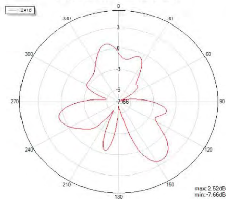
Phi=90 freq=2416MHz
