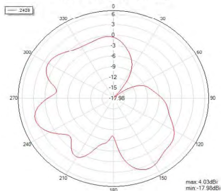
Phi=0 freq=2428MHz
