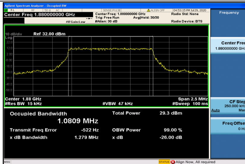
Band2-1.4MHz-QPSK-18900-6RB#0-1.0809
