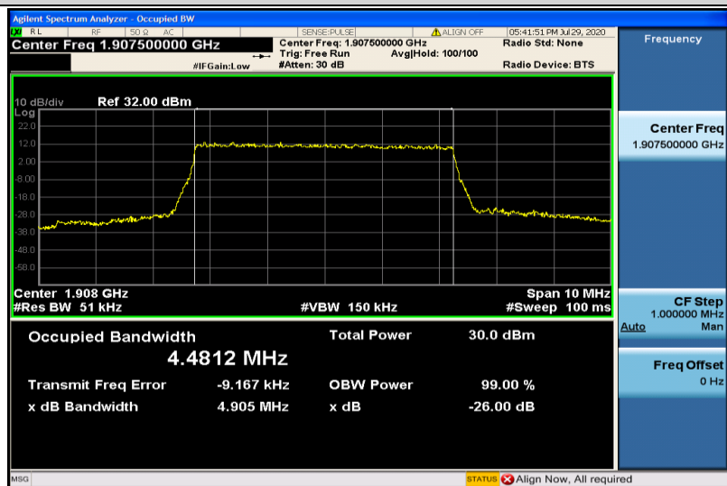
Band2-5MHz-QPSK-19175-25RB#0-4.4812
