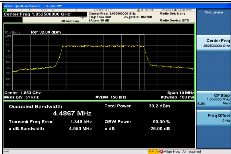
Band2-5MHz-QPSK-18625-25RB#0-4.4867
