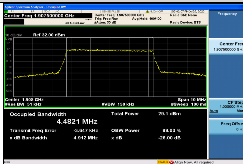
Band2-5MHz-16QAM-19175-25RB#0-4.4821
