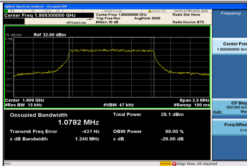
Band2-1.4MHz-16QAM-19193-6RB#0-1.0782
