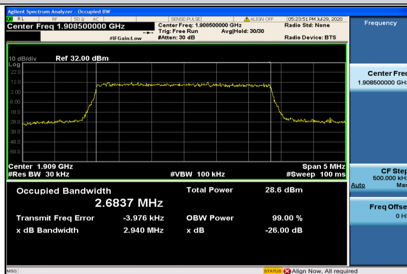
Band2-3MHz-16QAM-19185-15RB#0-2.6837
