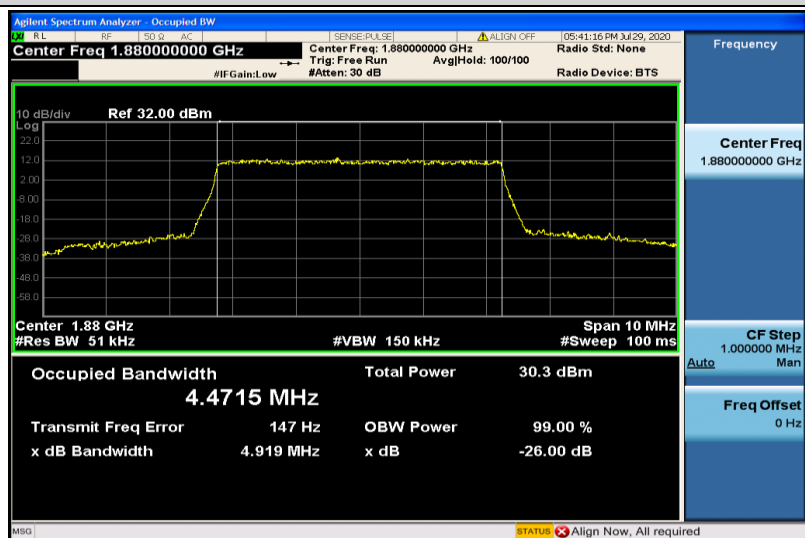
Band2-5MHz-QPSK-18900-25RB#0-4.4715
