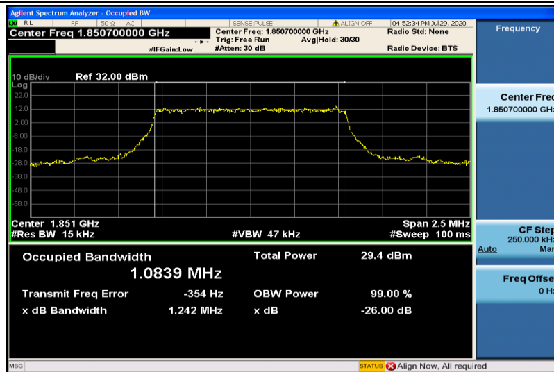
Band2-1.4MHz-QPSK-18607-6RB#0-1.0839
