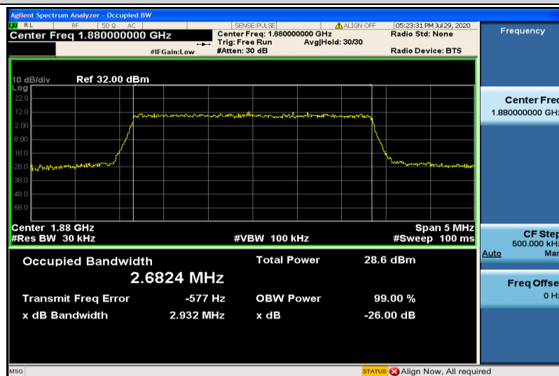
Band2-3MHz-16QAM-18900-15RB#0-2.6824
