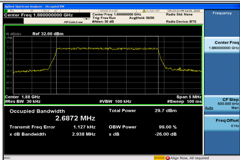
Band2-3MHz-QPSK-18900-15RB#0-2.6872
