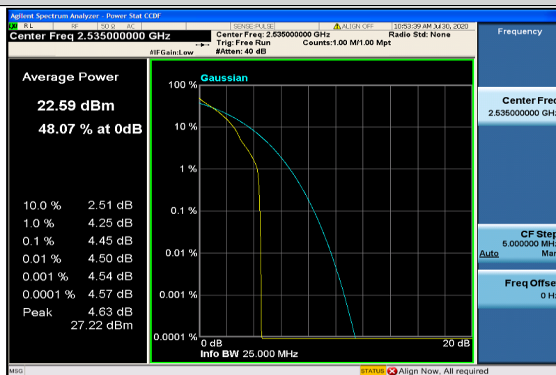
Band7-15MHz-QPSK-21100-1RB#0
