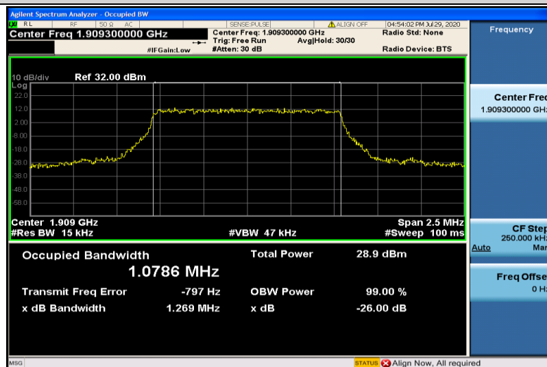
Band2-1.4MHz-QPSK-19193-6RB#0-1.0786
