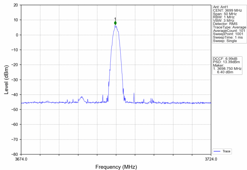
n78d_30kHz_SISO_NTNV_20MHz_DFT-s-OFDM_64_QAM_3690MHz_Edge_1RB_Right
