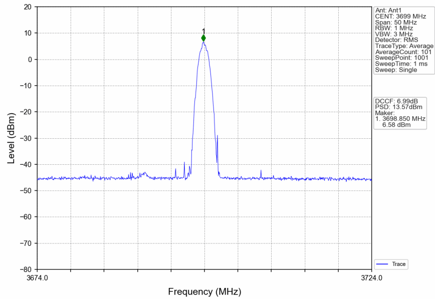
n78d_30kHz_SISO_NTNV_20MHz_DFT-s-OFDM_PI/2_BPSK_3690MHz_Edge_1RB_Right
