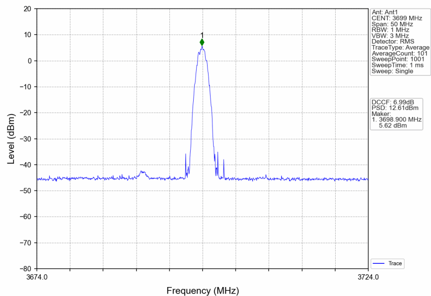
n78d_30kHz_SISO_NTNV_20MHz_DFT-s-OFDM_16_QAM_3690MHz_Edge_1RB_Right
