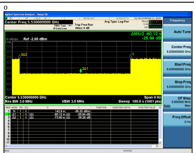
Initial CAC – 80MHz Bandwidth – 5530MHz
