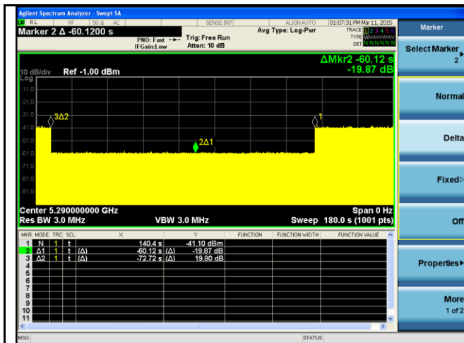
Initial CAC – 80MHz Bandwidth – 5290MHz
