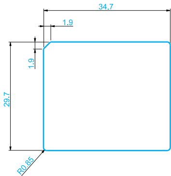
Die-line
