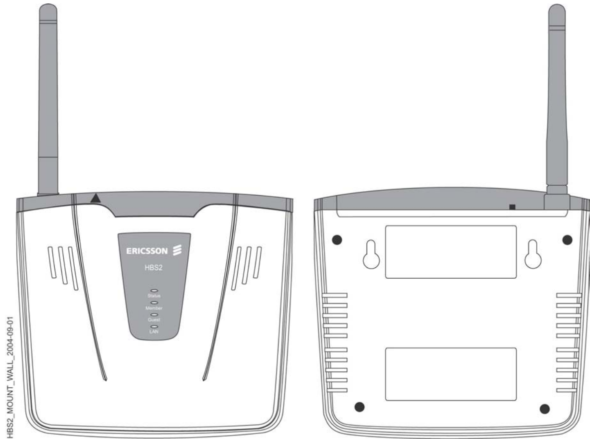
Figure 2 Wall mount. Front view to the left. Bottom view to the right. The Screw holes are 80 mm apart
