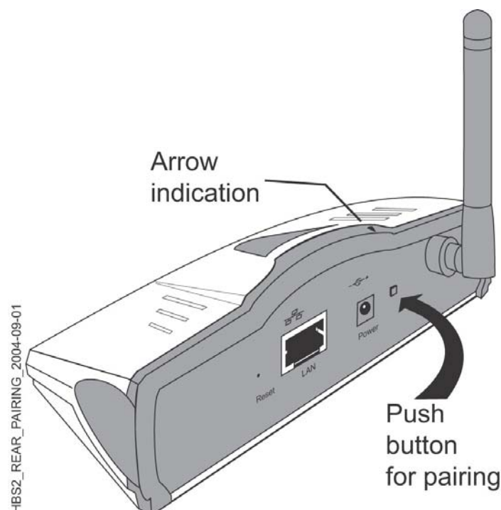
Figure 6 Press the Pairing button once for Member pairing and twice for Guest pairing
