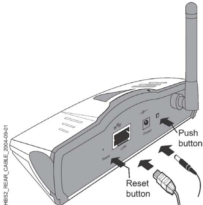
Figure 4 Cable connections
