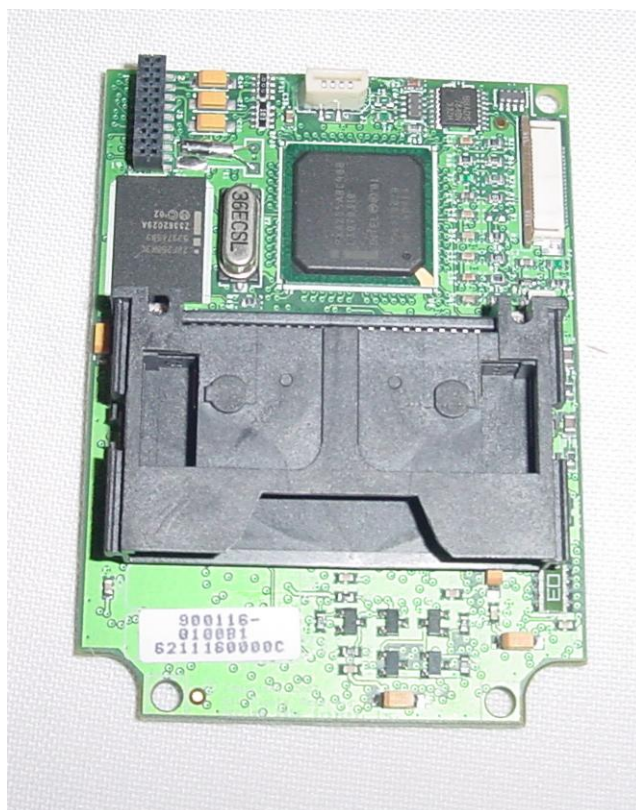
Internal Photo 9 – Win CE PCB Top View
