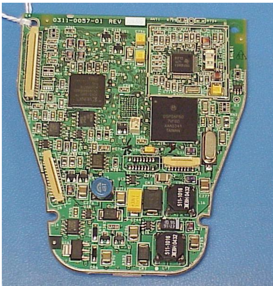
Internal Photo 8 – Pistol Processor PCB TopView
