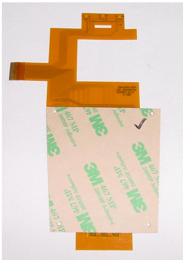
Internal Photo 2 – Keypad Interconnect Bottom View
