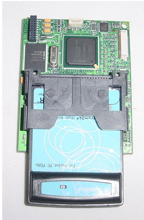
Internal Photo 11 – Win CE PCB and WLAN Card
