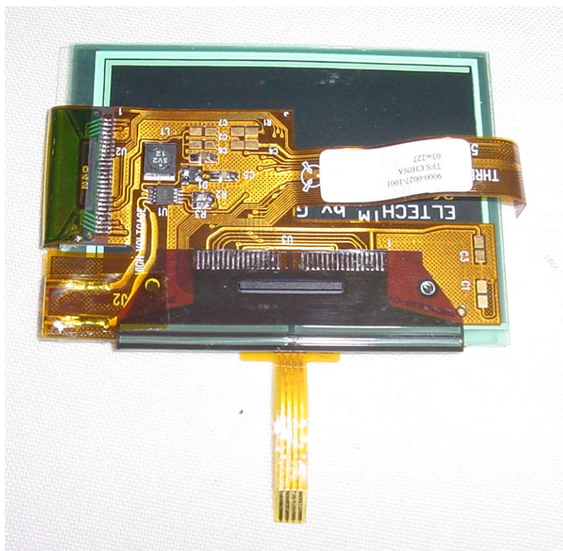
Internal Photo 3 – LCD Display Bottom View
