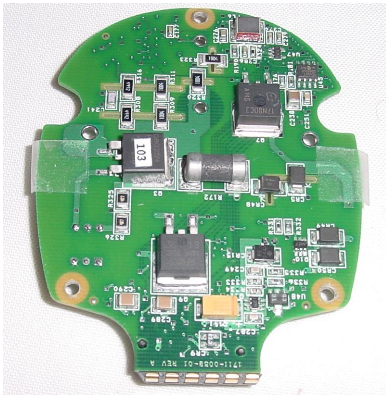
Internal Photo 5 – Pistol Power PCB Bottom View
