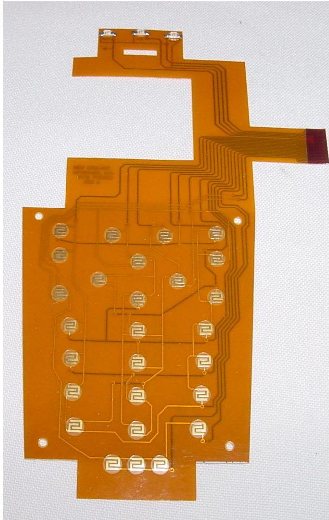
Internal Photo 1 – Keypad Interconnect Top View
